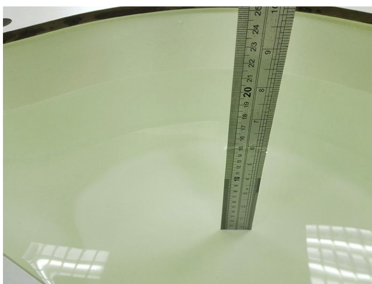
Photograph of the depth in the Body Phantom (2450MHz)
