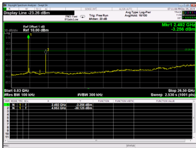
CH00 – 10th Harmonic of the fundamental frequency CH00 CH39 CH78
