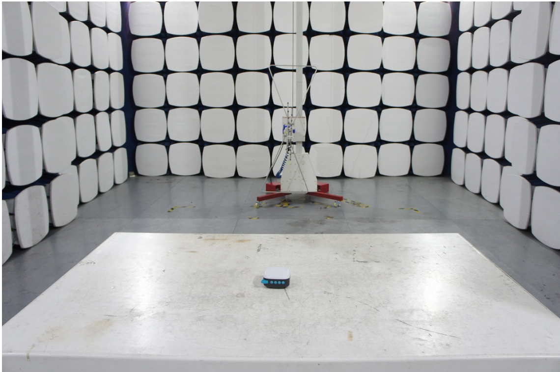
Test Setup Below 1GHz
