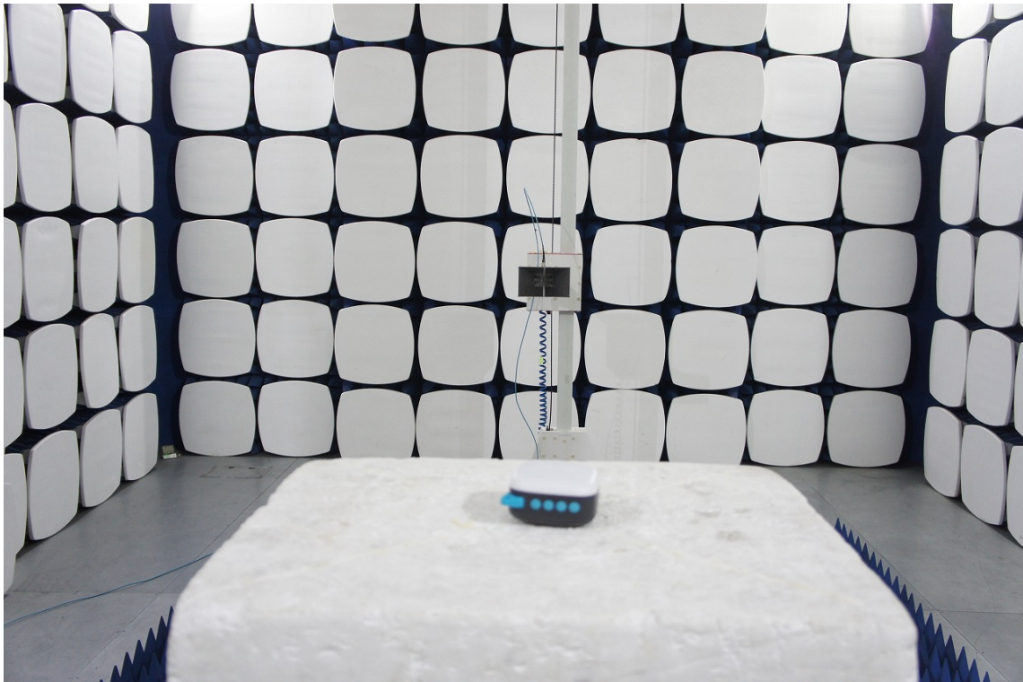
Above 1GHz
