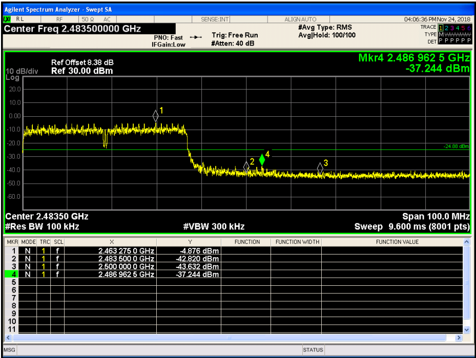
TX 11n40: Band edge-right side
