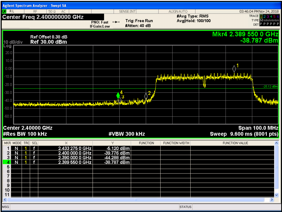
TX 11n40: Band edge-left side
