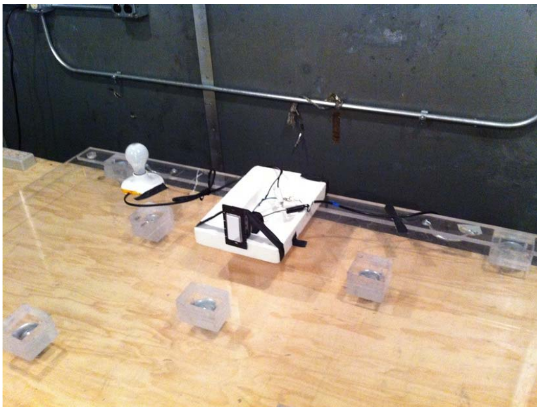
Mains Conducted Emission, Front
