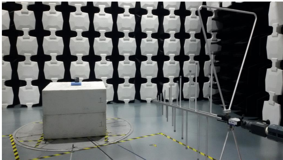
Description: Front view of Radiated Emission Test Setup (Below 1GHz)
