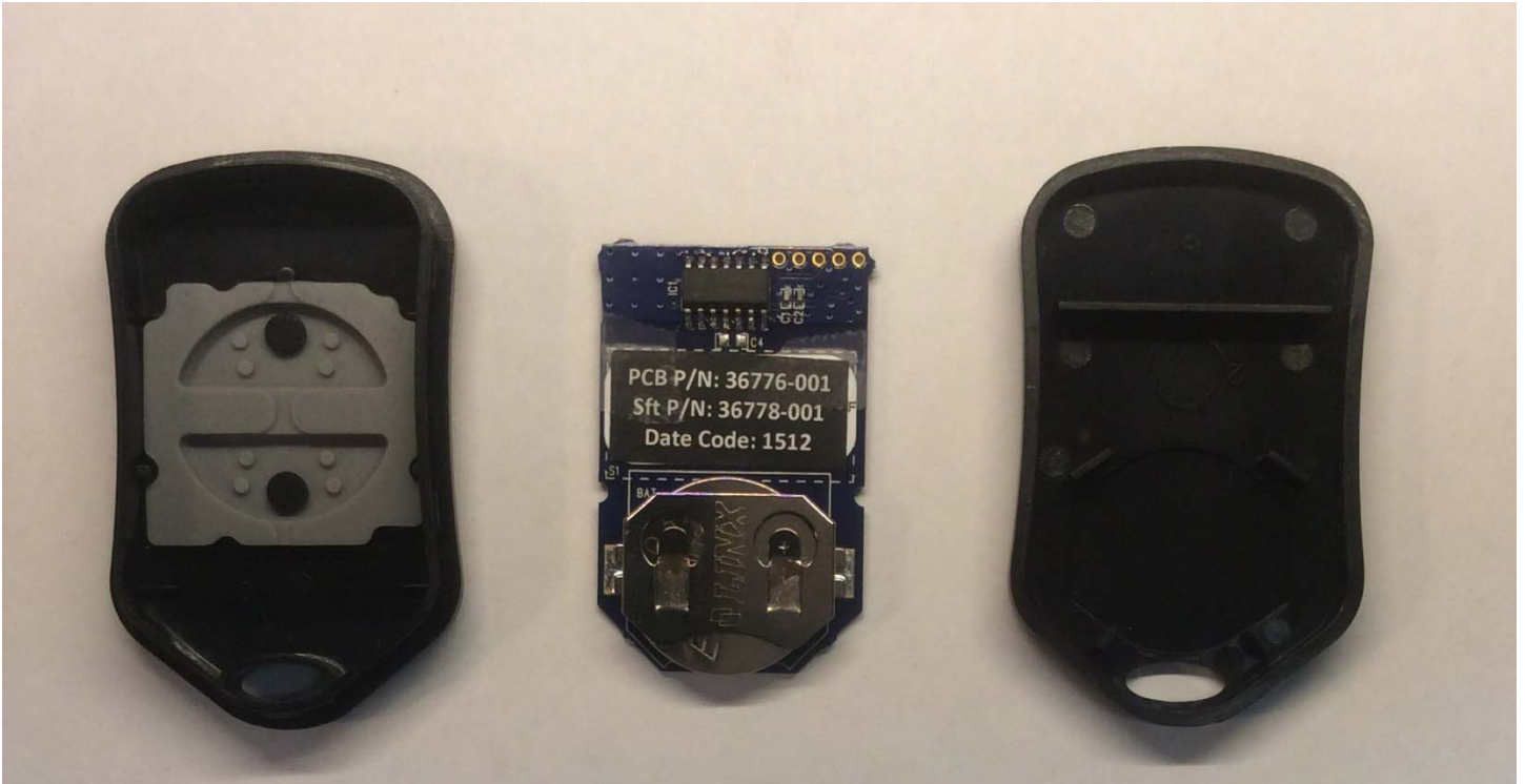
Figure 1: Internal Photo with Front PCB View
