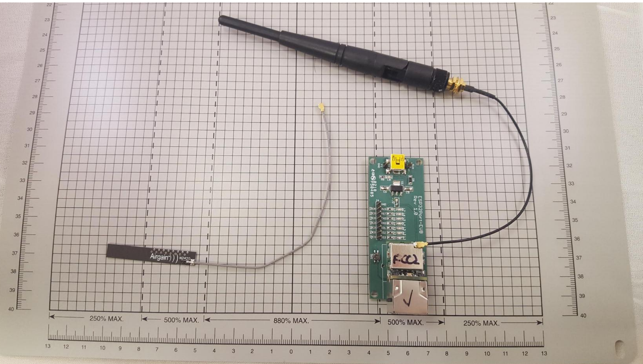
EUT mounted on Interface Board with Whip and PCB Antennas
