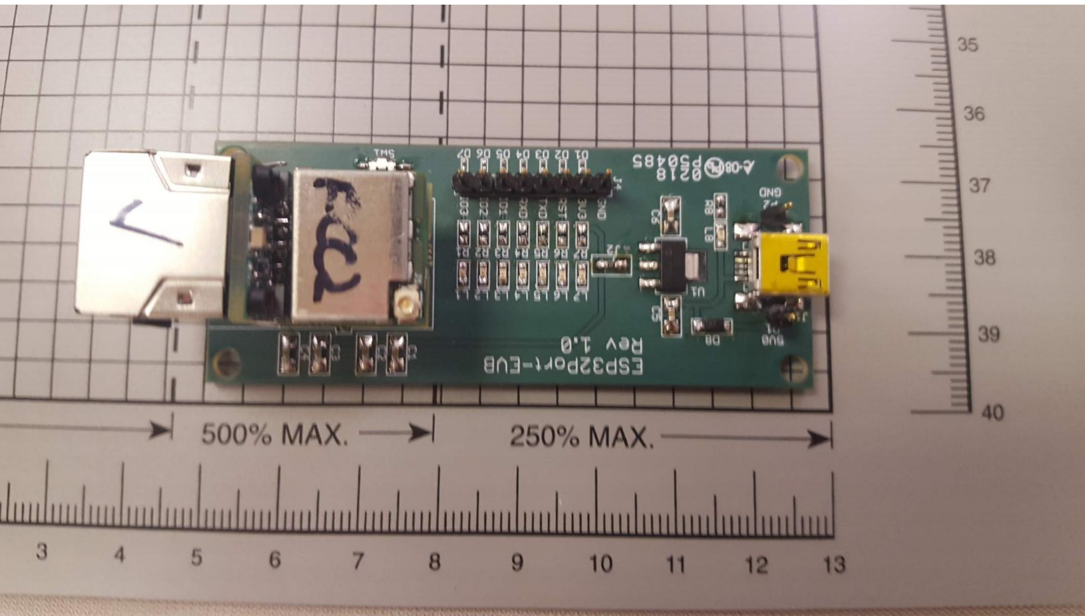
EUT on Interface Board
