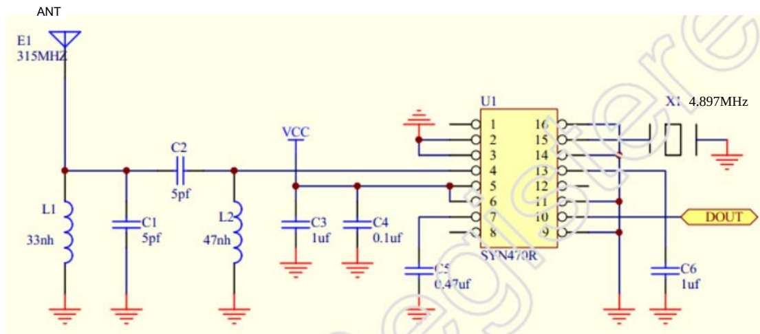
315MHz Receive Module circuit diagram
