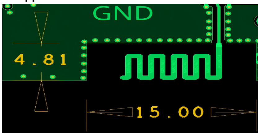
Planform
