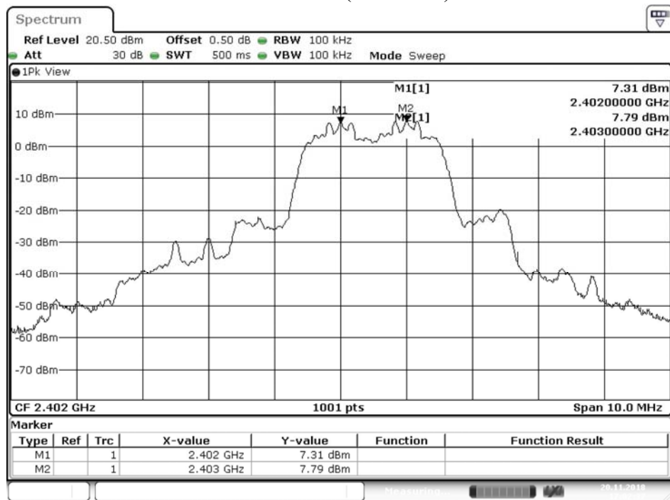
Channel 00 (2402MHz)
