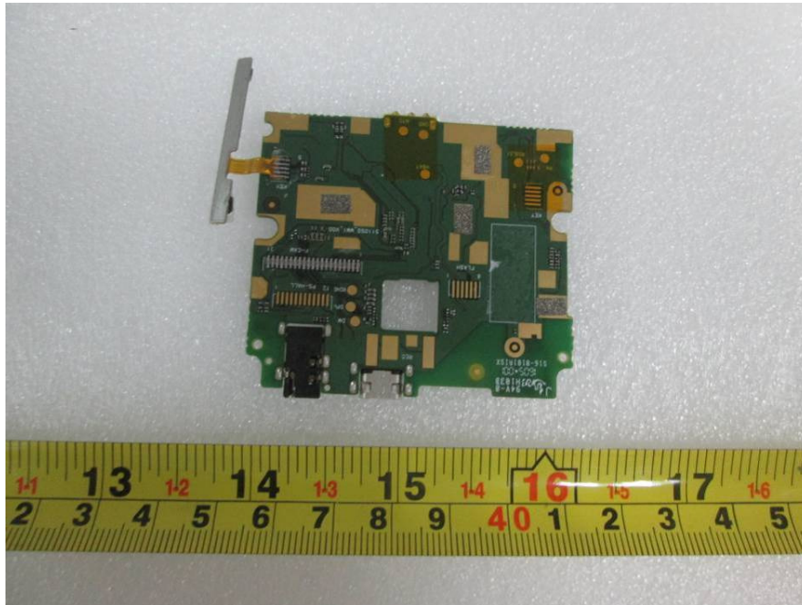
EUT – Main Board Bottom View (No Camera)
