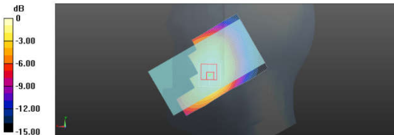
Left Head Cheek (WCDMA Band V Middle Channel)
