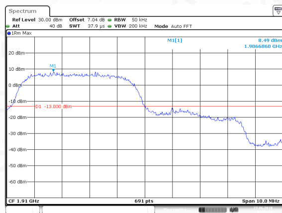
WCDMA 1900-HCH
