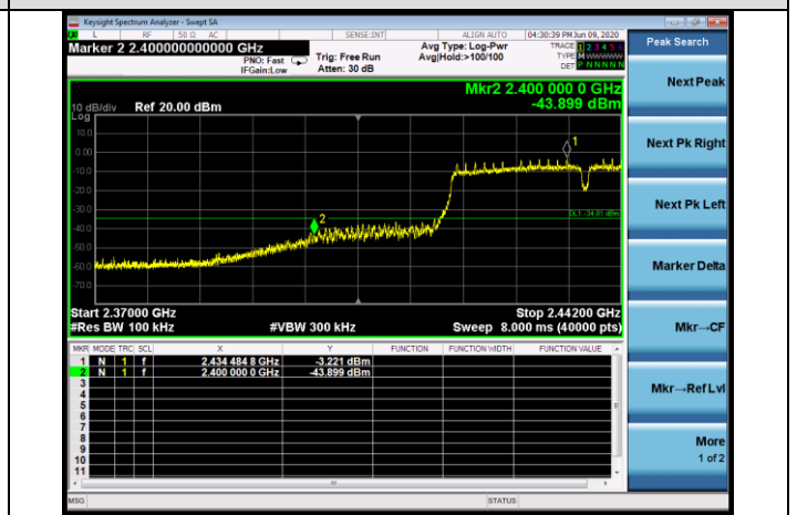
11nHT40-MCH
