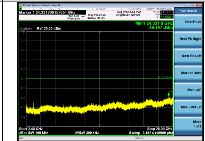
11nHT20-MCH
