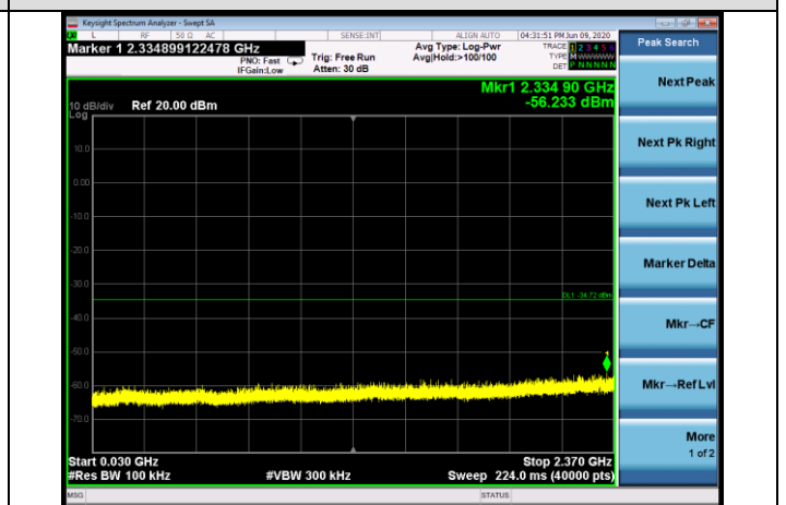
11nHT40-HCH
