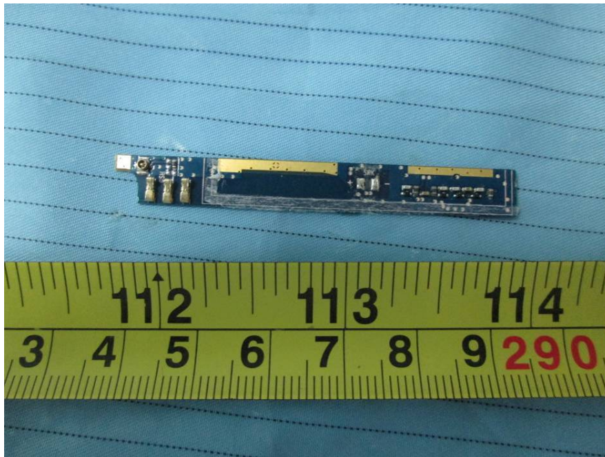
EUT – Sub Board Top Shielding off View
