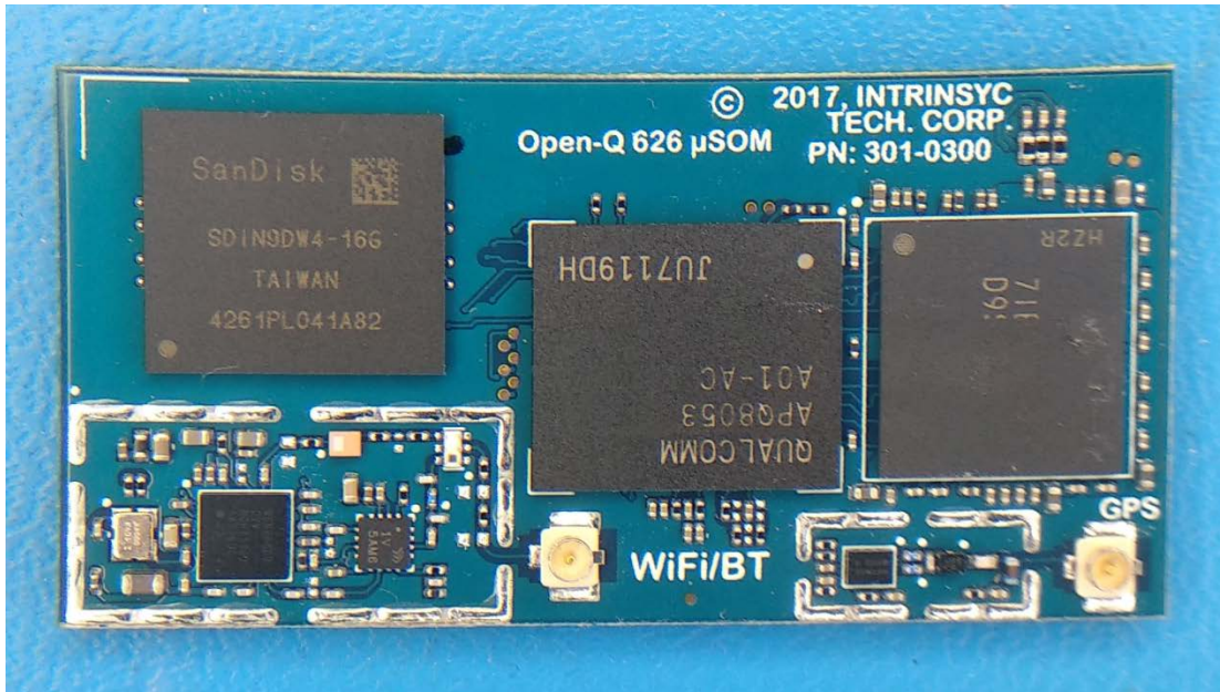
Top Side with RF Shield Covers Removed
