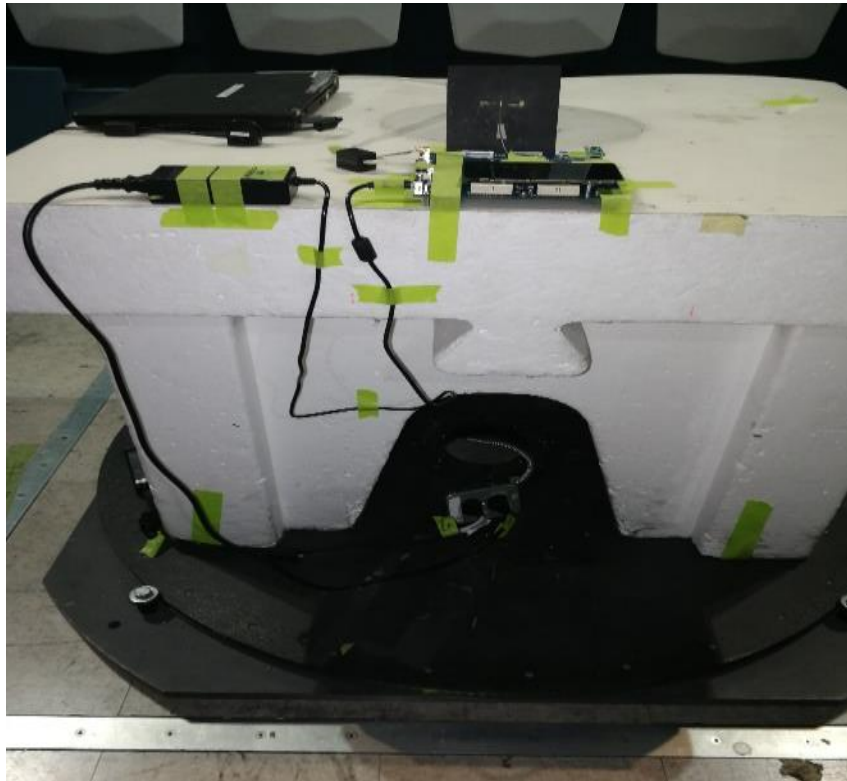
Figure R1: EUT Radiated Emissions Cable Layout
