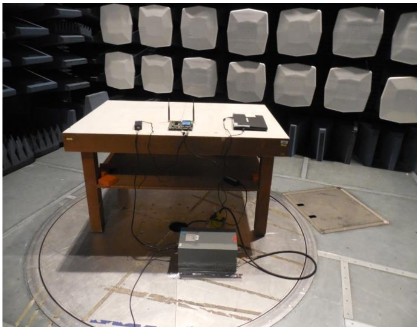
Figure R3: Conducted Emissions Test Setup
