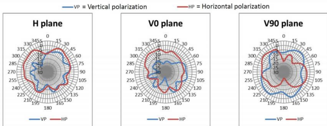
Figure 8 Niche Antenna 5GHz Operation
