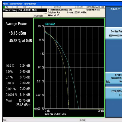
Band5-3MHz-16QAM-20525-15RB#0
