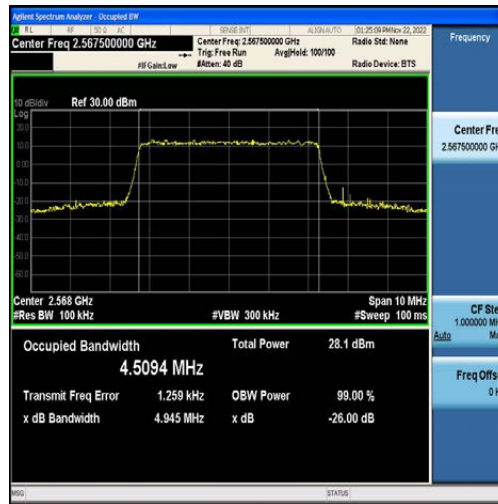
Band7-5MHz-16QAM-21425-25RB#0-4.5094
