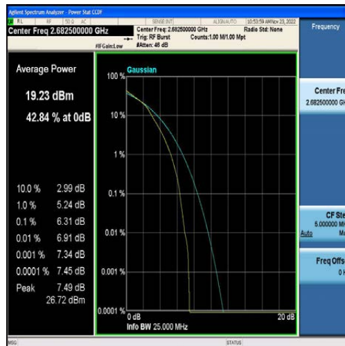
Band41-15MHz-16QAM-41515-75RB#0
