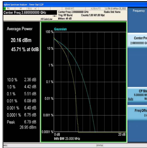
Band41-20MHz-QPSK-41490-100RB#0
