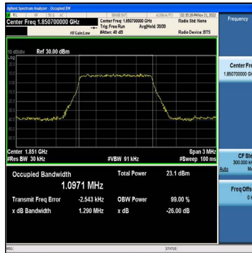
Band2-1.4MHz-QPSK-18607-6RB#0-1.0971
