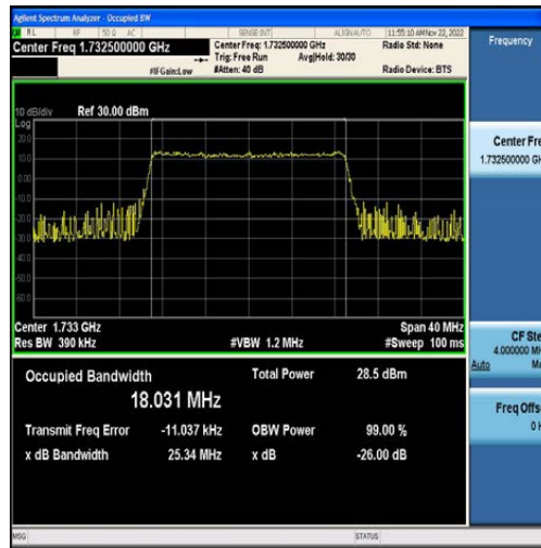
Band4-20MHz-QPSK-20175-100RB#0-18.031
