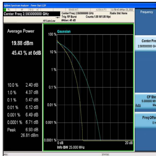
Band41-20MHz-QPSK-40620-100RB#0
