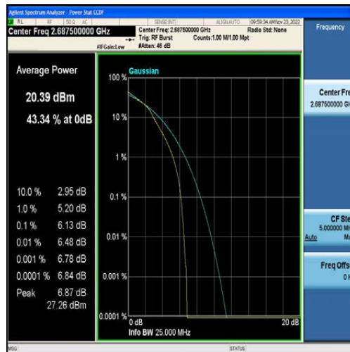
Band41-5MHz-16QAM-41565-25RB#0
