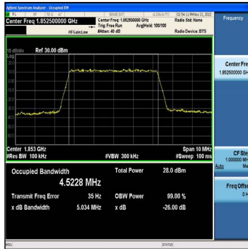
Band2-5MHz-QPSK-18625-25RB#0-4.5228
