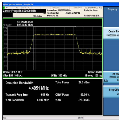
Band5-5MHz-16QAM-20525-25RB#0-4.4851
