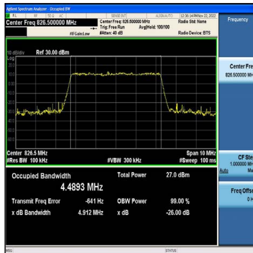
Band5-5MHz-16QAM-20425-25RB#0-4.4893
