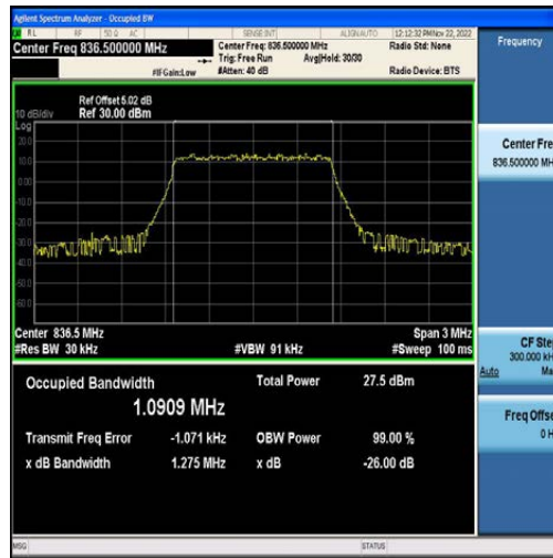
Band5-1.4MHz-QPSK-20525-6RB#0-1.0909
