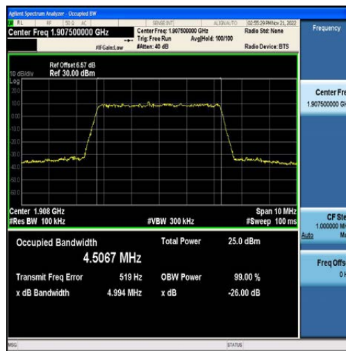
Band2-5MHz-16QAM-19175-25RB#0-4.5067
