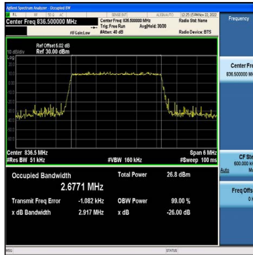
Band5-3MHz-16QAM-20525-15RB#0-2.6771
