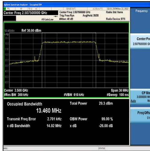
Band7-15MHz-QPSK-20825-75RB#0-13.460
