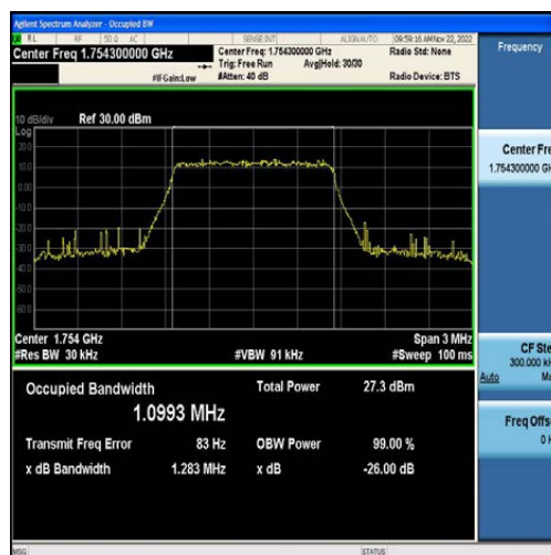
Band4-1.4MHz-QPSK-20393-6RB#0-1.0993
