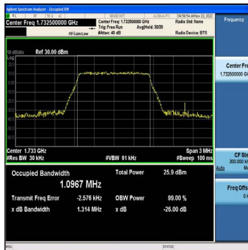
Band4-1.4MHz-16QAM-20175-6RB#0-1.0967
