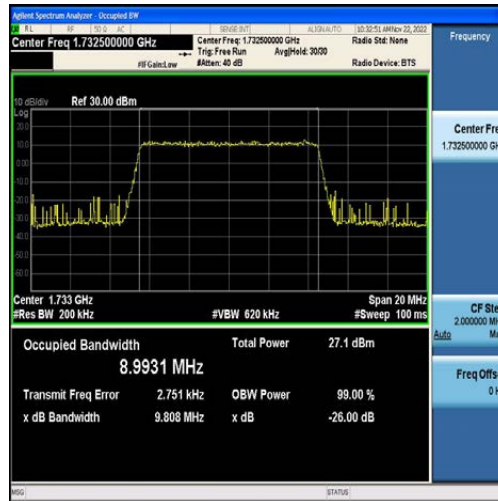
Band4-10MHz-16QAM-20175-50RB#0-8.9931
