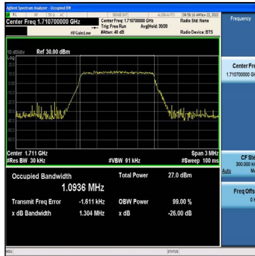
Band4-1.4MHz-QPSK-19957-6RB#0-1.0936
