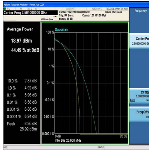
Band41-10MHz-16QAM-39700-50RB#0
