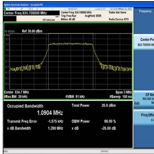
Band5-1.4MHz-QPSK-20407-6RB#0-1.0904
