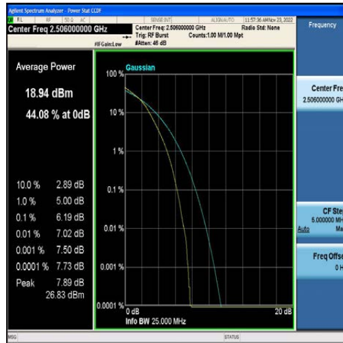
Band41-20MHz-16QAM-39750-100RB#0
