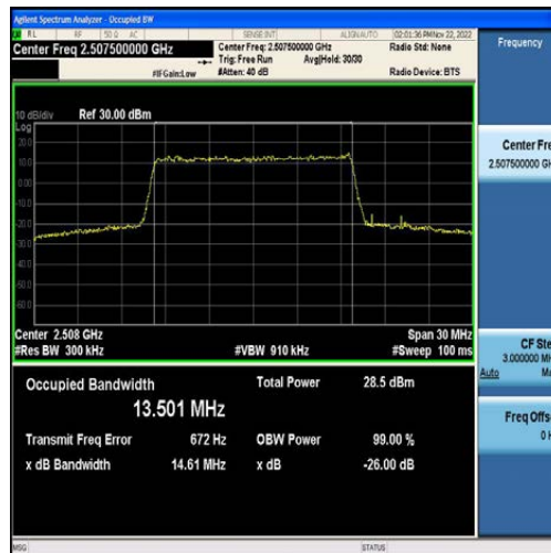
Band7-15MHz-16QAM-20825-75RB#0-13.501
