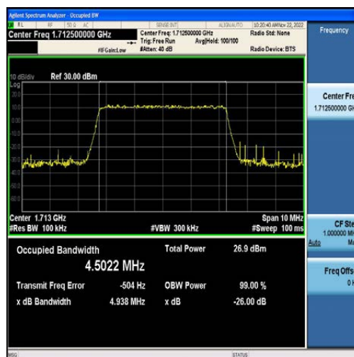
Band4-5MHz-16QAM-19975-25RB#0-4.5022
