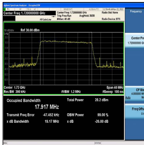
Band4-20MHz-QPSK-20050-100RB#0-17.917
