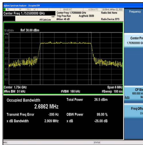
Band4-3MHz-16QAM-20385-15RB#0-2.6862
