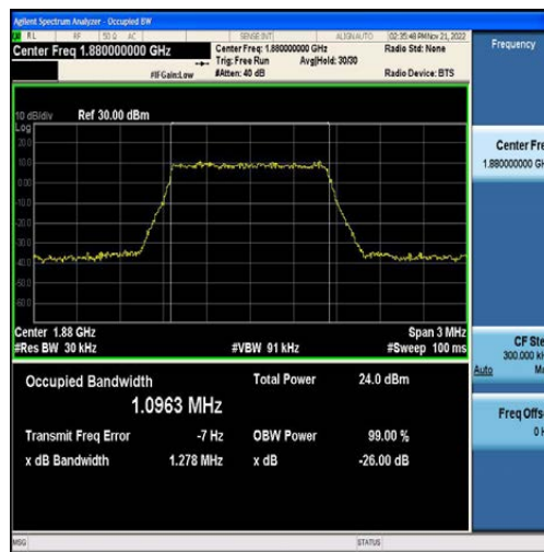
Band2-1.4MHz-QPSK-18900-6RB#0-1.0963
