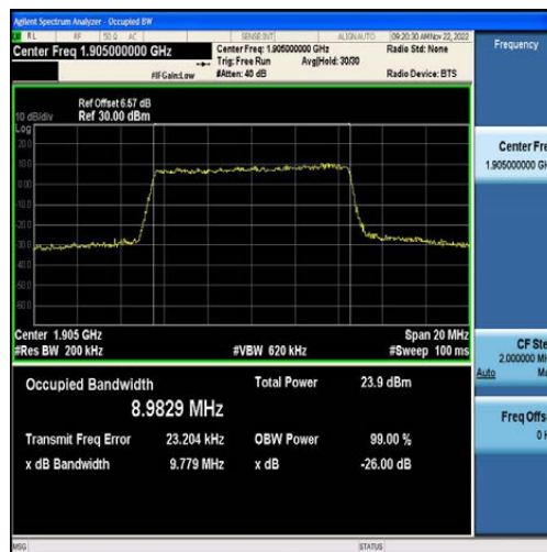
Band2-10MHz-QPSK-19150-50RB#0-8.9829
