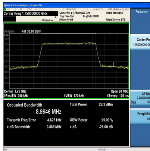
Band4-10MHz-QPSK-20350-50RB#0-8.9646
