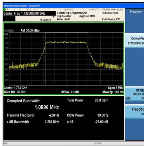
Band4-1.4MHz-QPSK-20175-6RB#0-1.0896
