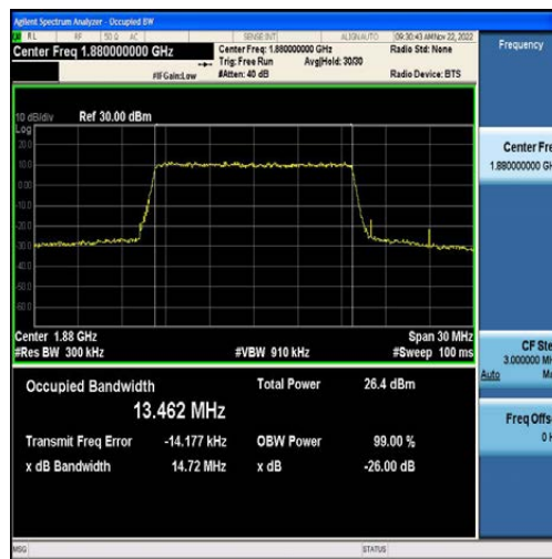
Band2-15MHz-QPSK-18900-75RB#0-13.462
