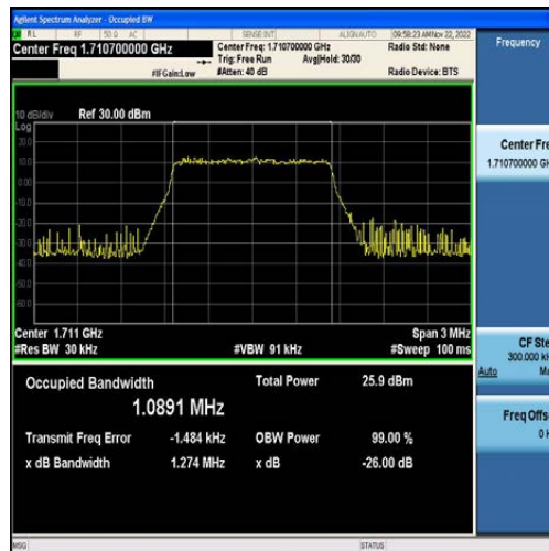
Band4-1.4MHz-16QAM-19957-6RB#0-1.0891
