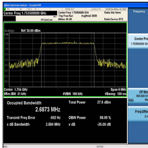
Band4-3MHz-QPSK-20385-15RB#0-2.6873
