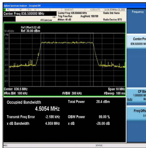
Band5-5MHz-QPSK-20525-25RB#0-4.5054
