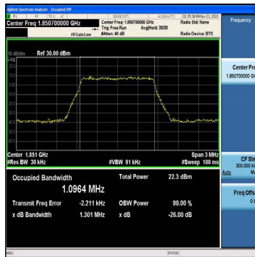
Band2-1.4MHz-16QAM-18607-6RB#0-1.0964
