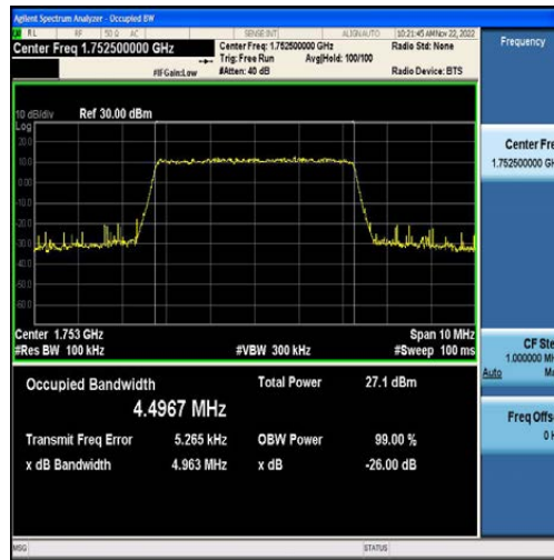
Band4-5MHz-16QAM-20375-25RB#0-4.4967
