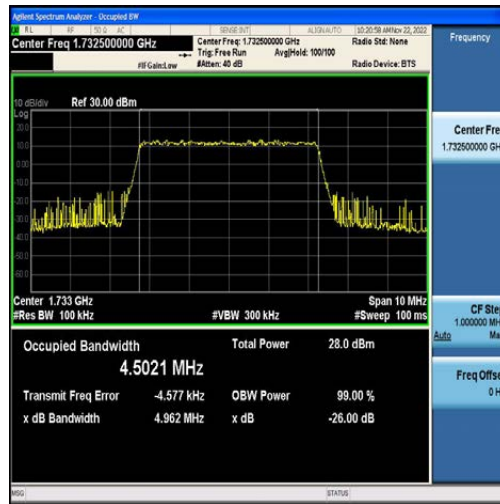
Band4-5MHz-QPSK-20175-25RB#0-4.5021
