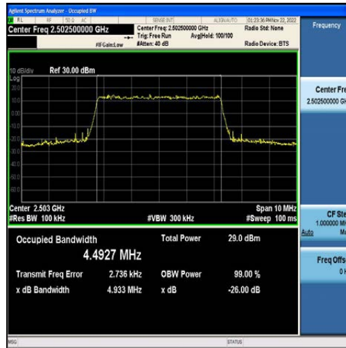
Band7-5MHz-QPSK-20775-25RB#0-4.4927
