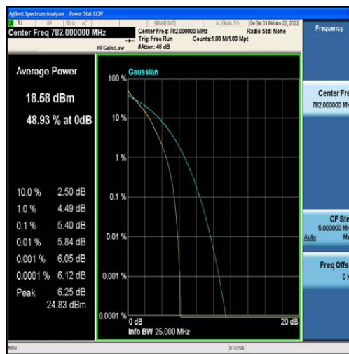
Band13-5MHz-QPSK-23230-25RB#0
