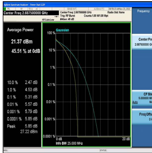
Band41-5MHz-QPSK-41565-25RB#0
