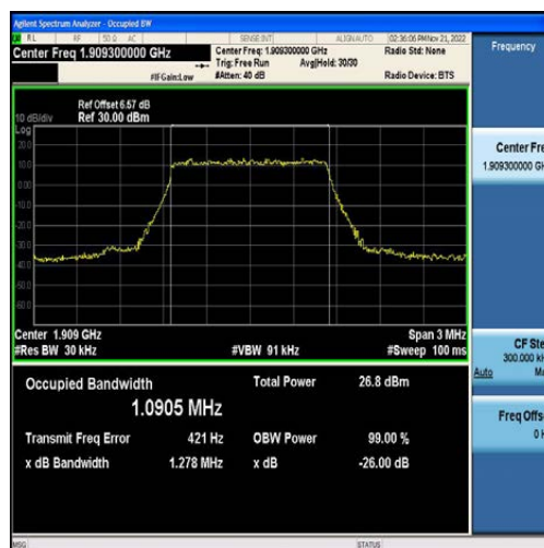
Band2-1.4MHz-QPSK-19193-6RB#0-1.0905
