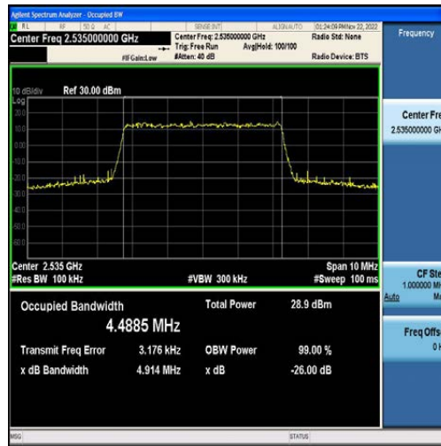
Band7-5MHz-QPSK-21100-25RB#0-4.4885
