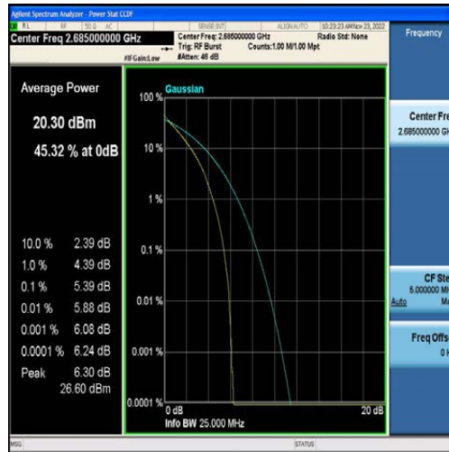
Band41-10MHz-QPSK-41540-50RB#0
