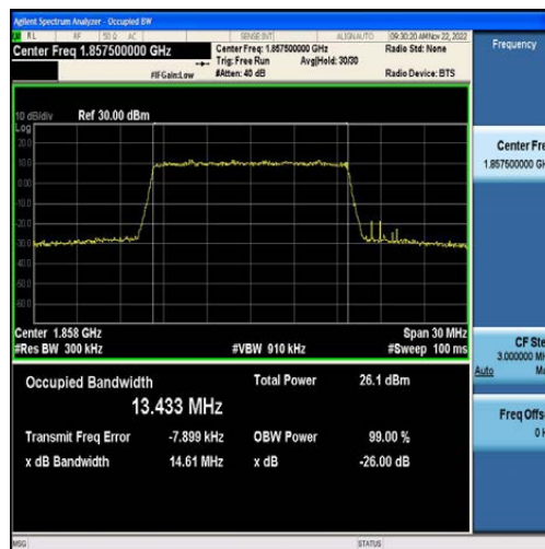
Band2-15MHz-16QAM-18675-75RB#0-13.433
