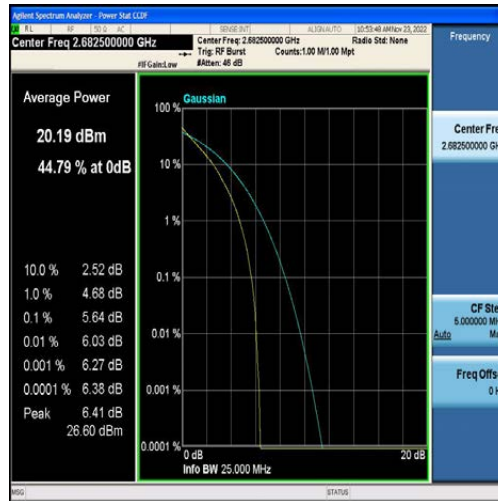
Band41-15MHz-QPSK-41515-75RB#0
