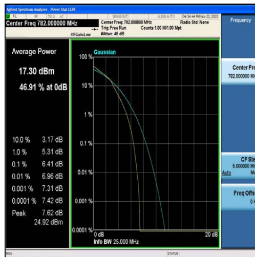
Band13-5MHz-16QAM-23230-25RB#0
