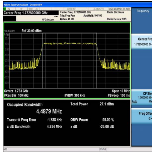
Band4-5MHz-16QAM-20175-25RB#0-4.4879
