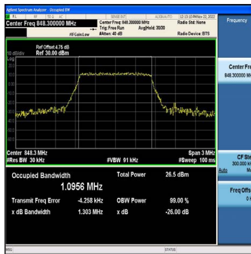
Band5-1.4MHz-16QAM-20643-6RB#0-1.0956
