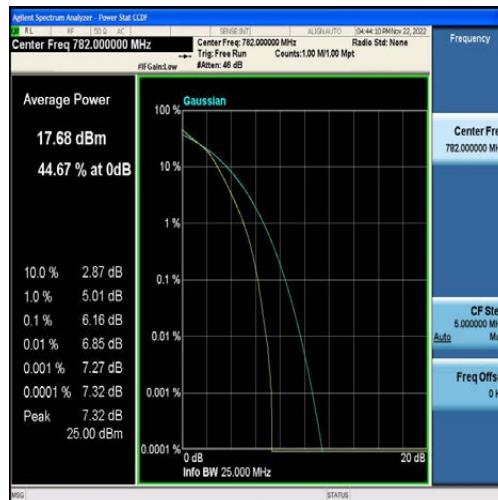
Band13-10MHz-16QAM-23230-50RB#0
