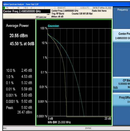
Band41-5MHz-QPSK-39675-25RB#0
