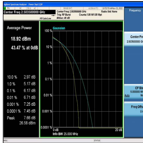
Band41-15MHz-16QAM-39725-75RB#0
