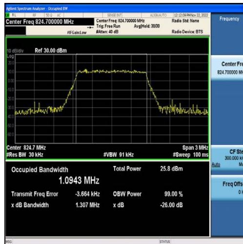
Band5-1.4MHz-16QAM-20407-6RB#0-1.0943
