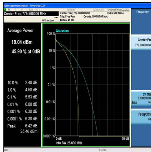
Band13-5MHz-QPSK-23205-25RB#0
