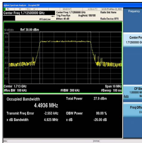
Band4-5MHz-QPSK-19975-25RB#0-4.4936
