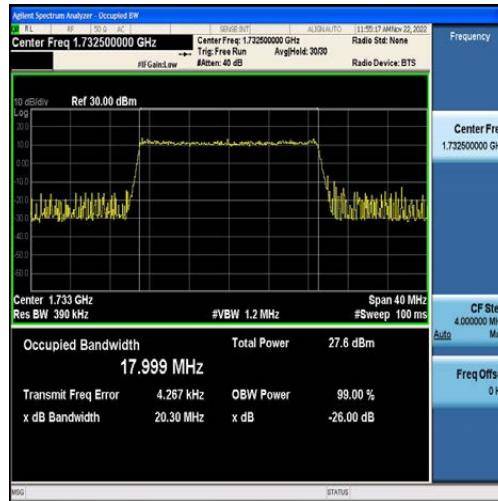
Band4-20MHz-16QAM-20175-100RB#0-17.999
