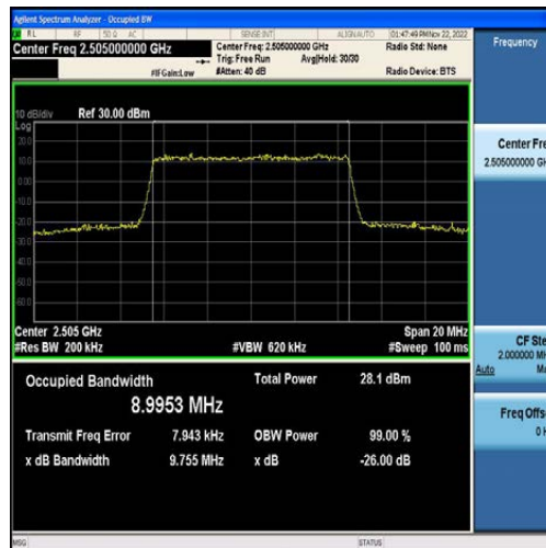
Band7-10MHz-16QAM-20800-50RB#0-8.9953
