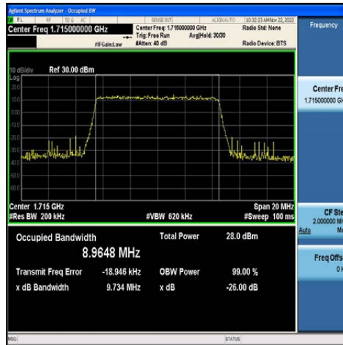
Band4-10MHz-QPSK-20000-50RB#0-8.9648
