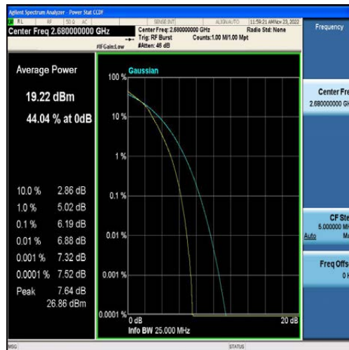
Band41-20MHz-16QAM-41490-100RB#0
