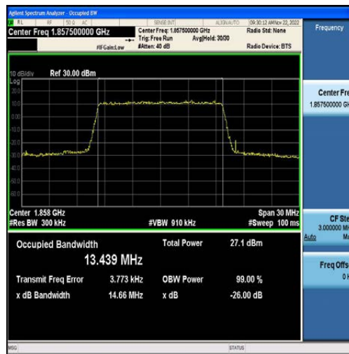
Band2-15MHz-QPSK-18675-75RB#0-13.439
