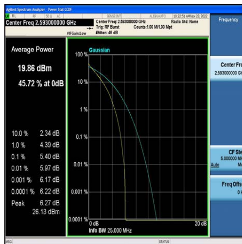
Band41-10MHz-QPSK-40620-50RB#0
