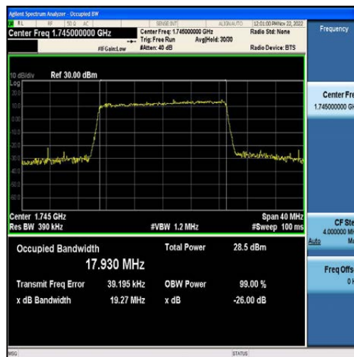
Band4-20MHz-QPSK-20300-100RB#0-17.930
