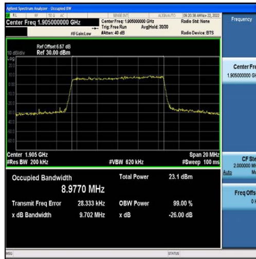
Band2-10MHz-16QAM-19150-50RB#0-8.9770
