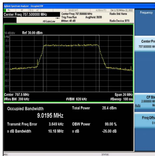
Band12-10MHz-QPSK-23095-50RB#0-9.0195
