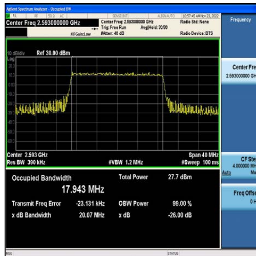
Band41-20MHz-16QAM-40620-100RB#0-17.943
