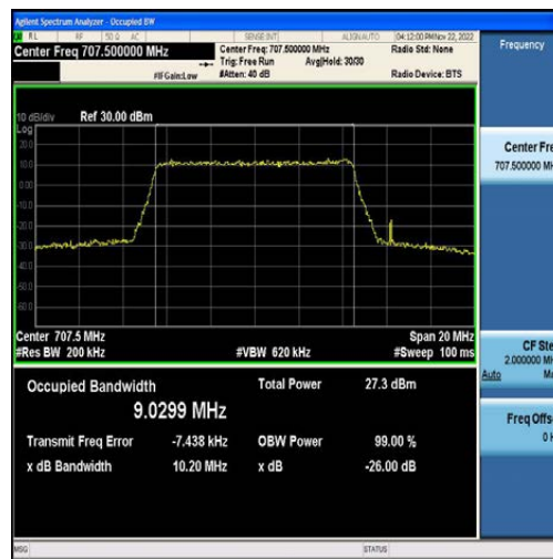
Band12-10MHz-16QAM-23095-50RB#0-9.0299
