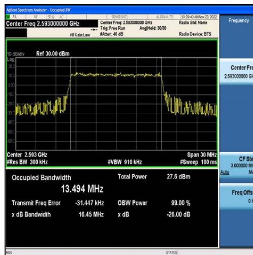
Band41-15MHz-16QAM-40620-75RB#0-13.494
