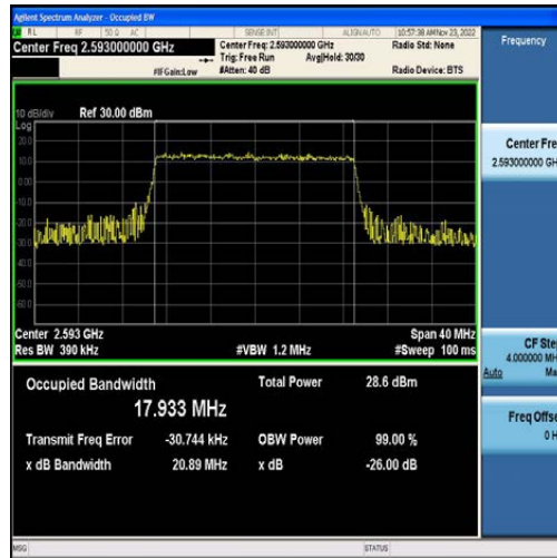
Band41-20MHz-QPSK-40620-100RB#0-17.933
