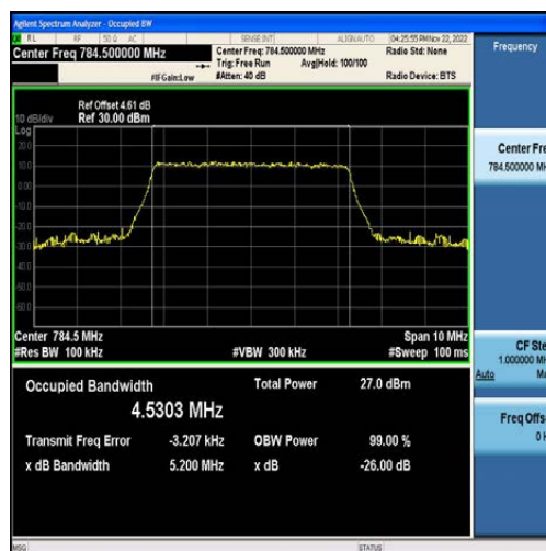
Band13-5MHz-16QAM-23255-25RB#0-4.5303
