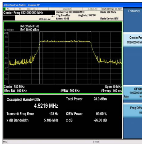
Band13-5MHz-QPSK-23230-25RB#0-4.5219
