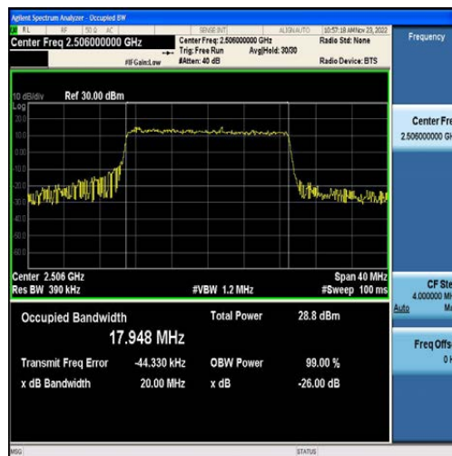
Band41-20MHz-QPSK-39750-100RB#0-17.948
