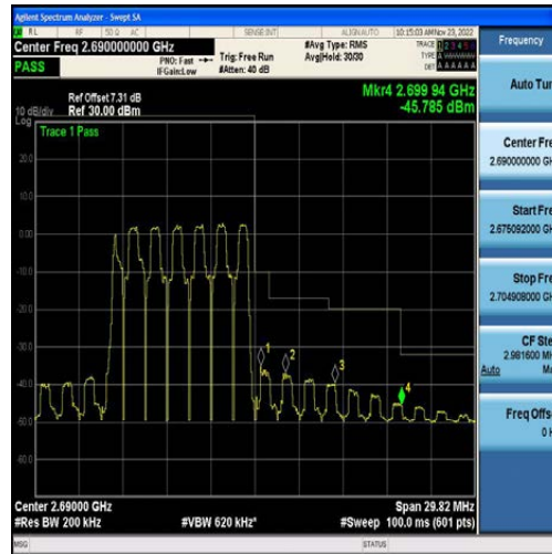
Band41-10MHz-16QAM-41540-50RB#0
