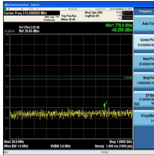
Band2-3MHz-QPSK-18615-15RB#0-Range1:30~1000MHz
