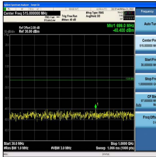
Band2-1.4MHz-16QAM-18900-6RB#0-Range1:30~1000MHz
