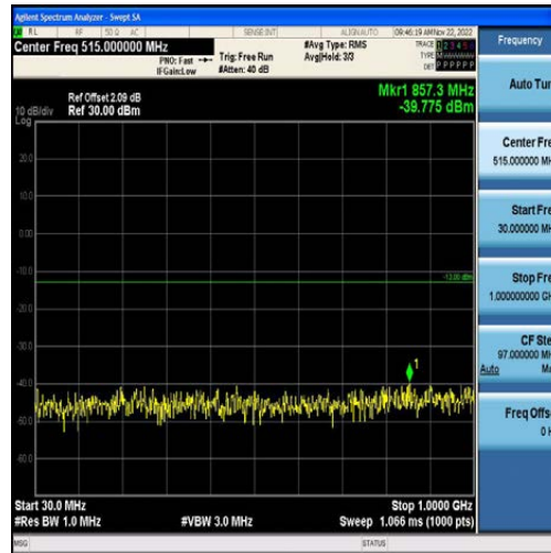
Band2-20MHz-16QAM-18900-100RB#0-Range1:30~1000MHz
