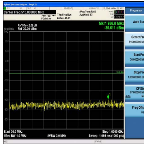
Band4-5MHz-QPSK-19975-25RB#0-Range1:30~1000MHz
