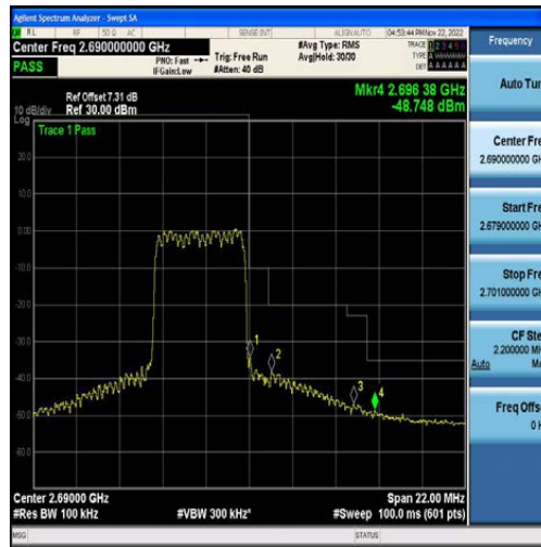
Band41-5MHz-16QAM-41565-25RB#0
