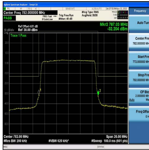
Band13-10MHz-QPSK-23230-50RB#0
