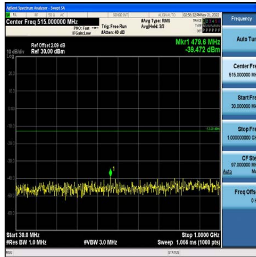
Band2-5MHz-QPSK-18625-25RB#0-Range1:30~1000MHz
