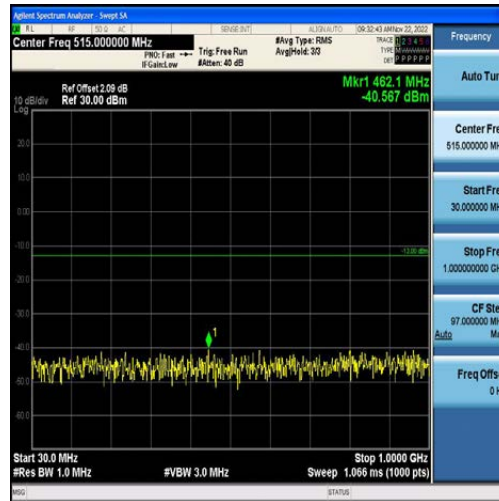
Band2-15MHz-QPSK-18675-75RB#0-Range1:30~1000MHz
