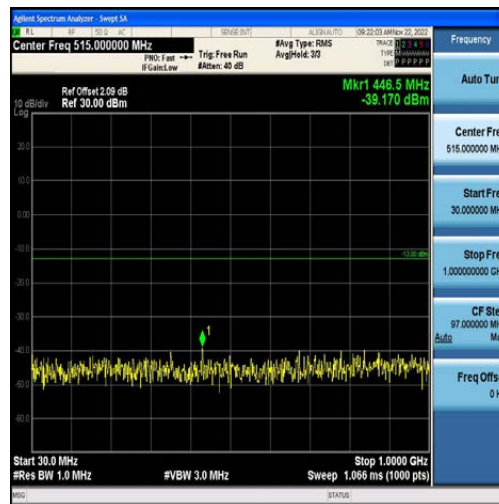
Band2-10MHz-QPSK-18650-50RB#0-Range1:30~1000MHz
