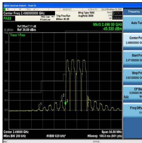
Band41-10MHz-16QAM-39700-50RB#0
