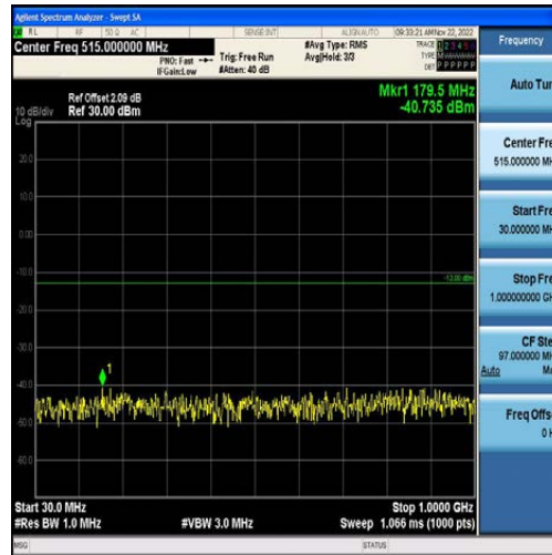
Band2-15MHz-16QAM-18900-75RB#0-Range1:30~1000MHz
