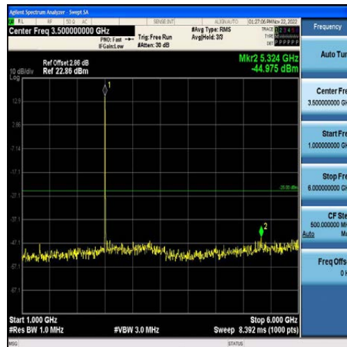
Band7-5MHz-16QAM-20775-25RB#0-Range2:1000~6000MHz
