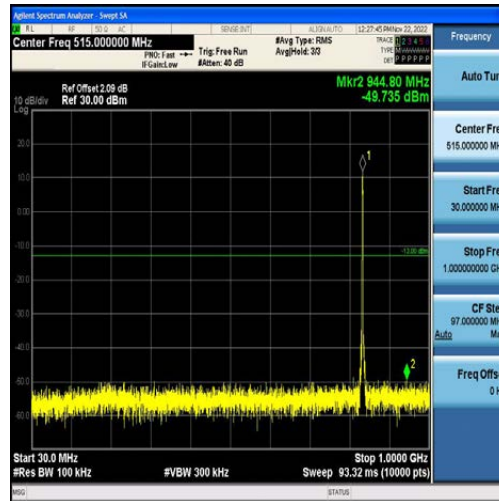
Band5-3MHz-16QAM-20525-15RB#0-Range1:30~1000MHz
