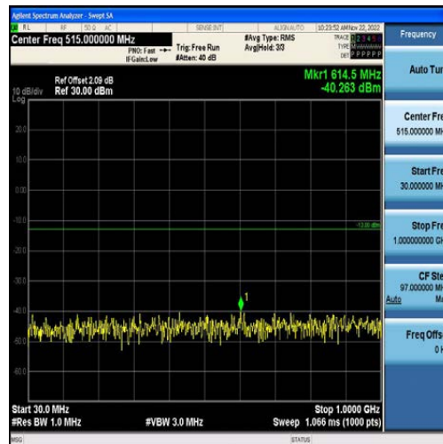
Band4-5MHz-16QAM-20375-25RB#0-Range1:30~1000MHz
