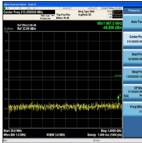
Band7-15MHz-16QAM-21100-75RB#0-Range1:30~1000MHz
