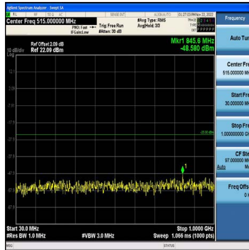
Band7-5MHz-16QAM-20775-25RB#0-Range1:30~1000MHz
