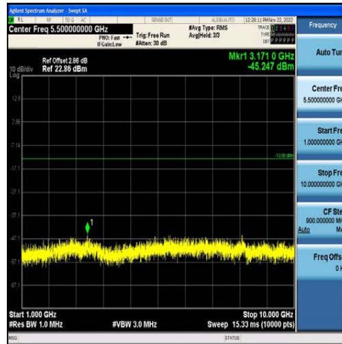
Band5-3MHz-QPSK-20635-15RB#0-Range2:1000~10000MHz
