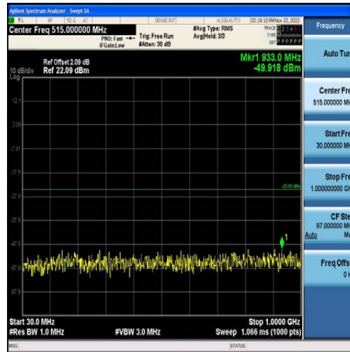
Band7-15MHz-QPSK-21375-75RB#0-Range1:30~1000MHz
