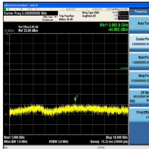
Band5-3MHz-16QAM-20525-15RB#0-Range2:1000~10000MHz
