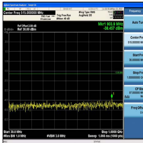
Band4-15MHz-16QAM-20325-75RB#0-Range1:30~1000MHz
