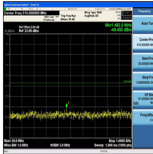
Band7-5MHz-QPSK-21100-25RB#0-Range1:30~1000MHz
