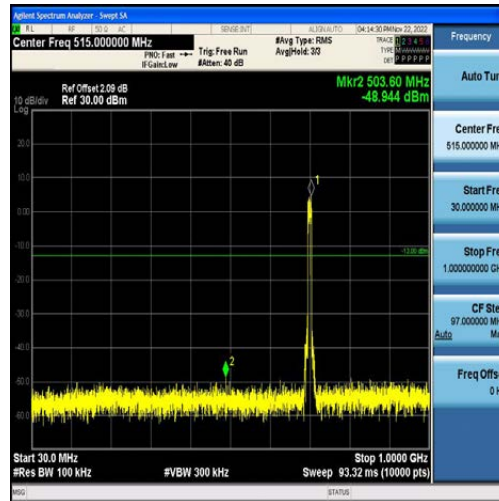
Band12-10MHz-16QAM-23095-50RB#0-Range1:30~1000MHz
