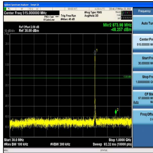
Band12-3MHz-16QAM-23095-15RB#0-Range1:30~1000MHz
