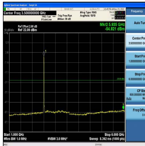
Band41-15MHz-16QAM-39725-75RB#0-Range2:1000~6000MHz
