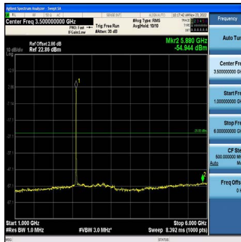
Band41-10MHz-16QAM-40620-50RB#0-Range2:1000~6000MHz
