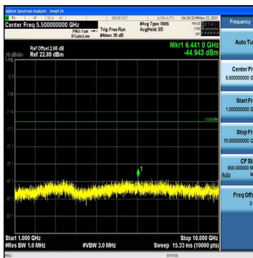
Band13-5MHz-16QAM-23255-25RB#0-Range2:1000~10000MHz
