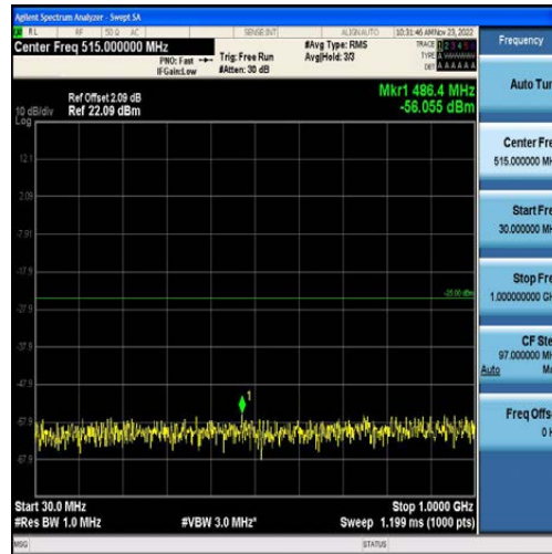
Band41-15MHz-QPSK-39725-75RB#0-Range1:30~1000MHz
