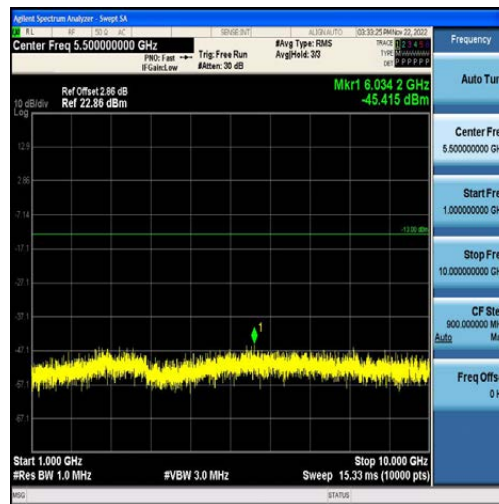
Band12-1.4MHz-QPSK-23173-6RB#0-Range2:1000~10000MHz
