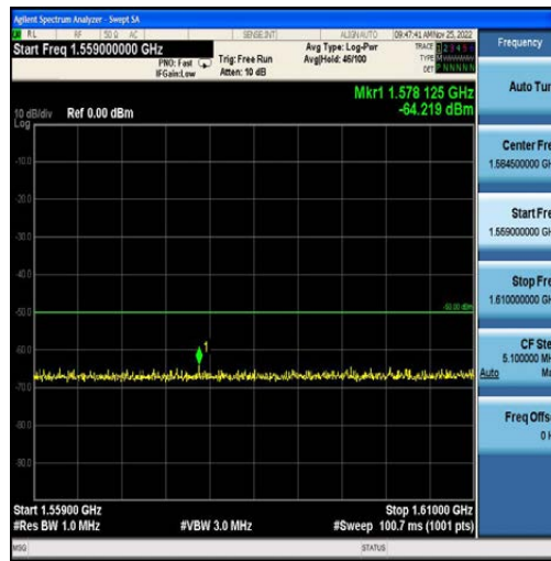
Band13-5MHz-QPSK-23230-25RB#0-Range3:1559~1610MHz
