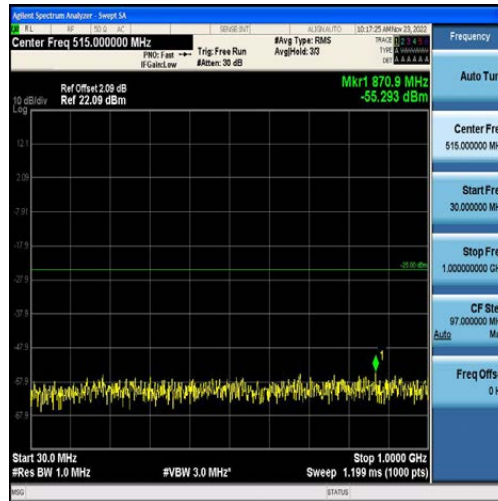
Band41-10MHz-QPSK-40620-50RB#0-Range1:30~1000MHz
