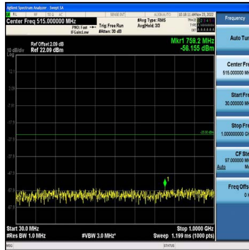
Band41-10MHz-16QAM-41540-50RB#0-Range1:30~1000MHz
