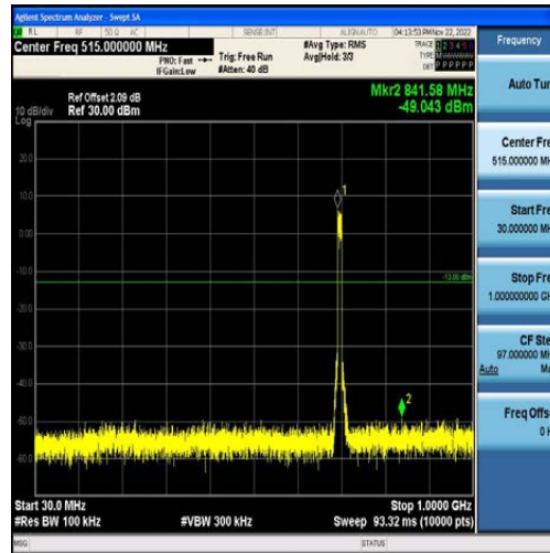
Band12-10MHz-QPSK-23060-50RB#0-Range1:30~1000MHz
