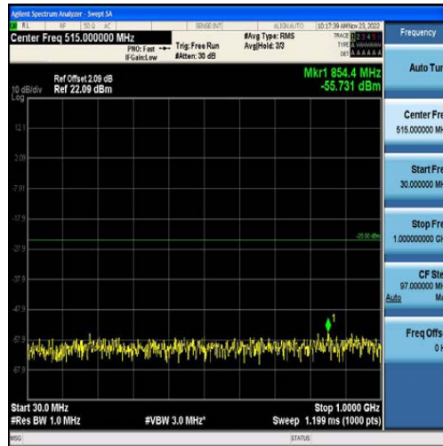
Band41-10MHz-16QAM-40620-50RB#0-Range1:30~1000MHz
