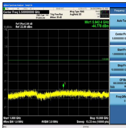
Band13-10MHz-16QAM-23230-50RB#0-Range2:1000~10000MHz
