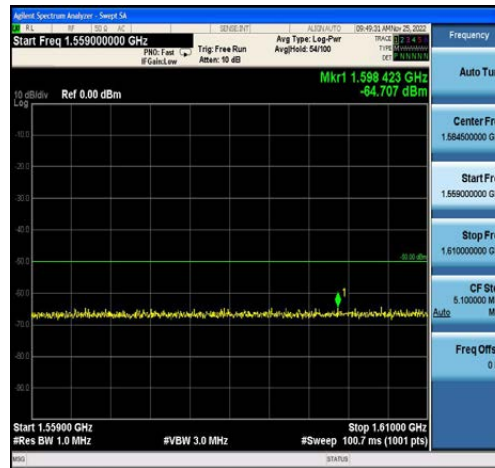
Band13-10MHz-16QAM-23230-50RB#0-Range3:1559~1610MHz
