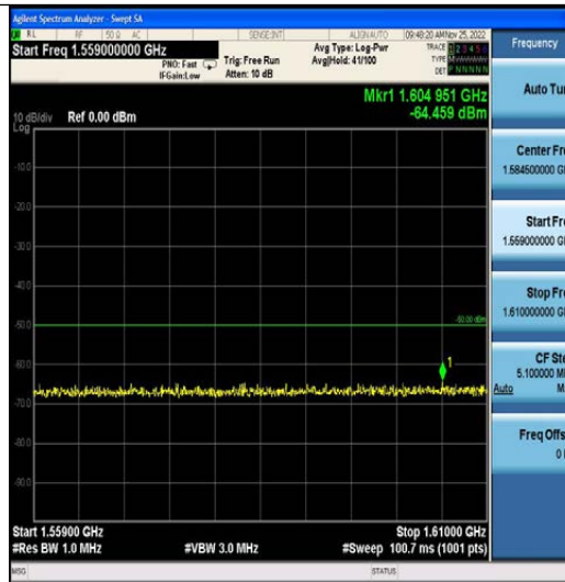
Band13-5MHz-16QAM-23255-25RB#0-Range3:1559~1610MHz
