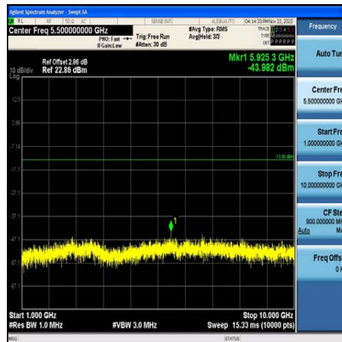
Band12-10MHz-16QAM-23095-50RB#0-Range2:1000~10000MHz
