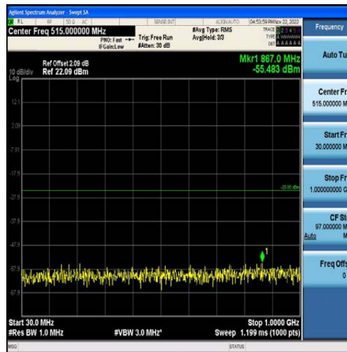
Band41-5MHz-QPSK-39675-25RB#0-Range1:30~1000MHz
