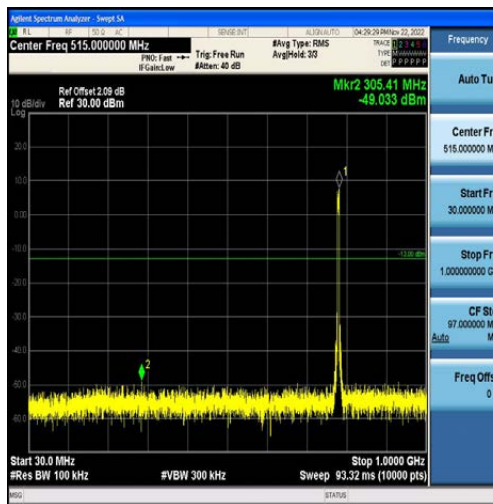
Band13-5MHz-16QAM-23255-25RB#0-Range1:30~1000MHz
