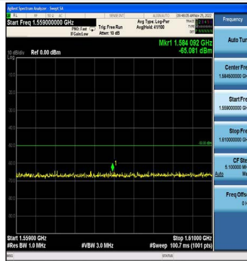
Band13-5MHz-QPSK-23255-25RB#0-Range3:1559~1610MHz
