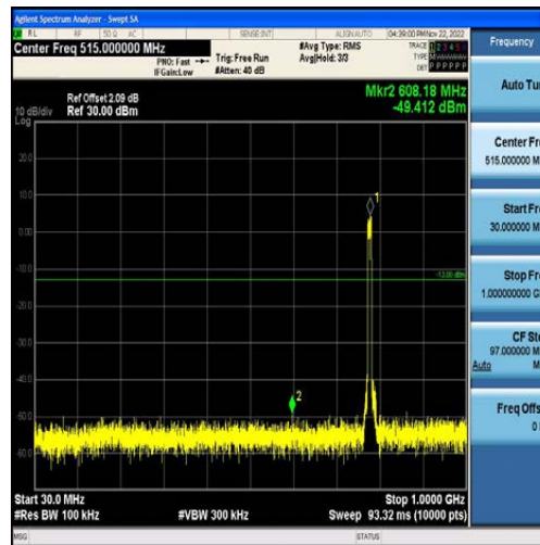
Band13-10MHz-16QAM-23230-50RB#0-Range1:30~1000MHz
