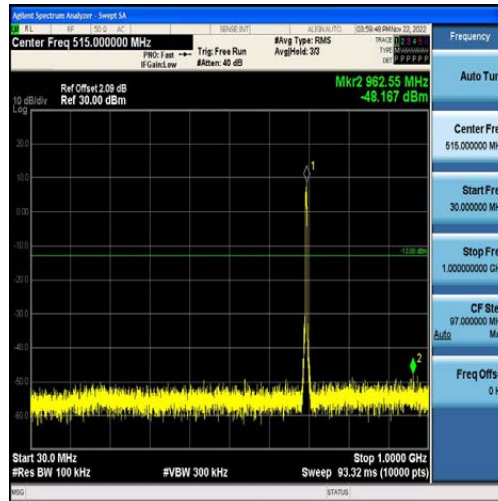
Band12-5MHz-QPSK-23035-25RB#0-Range1:30~1000MHz
