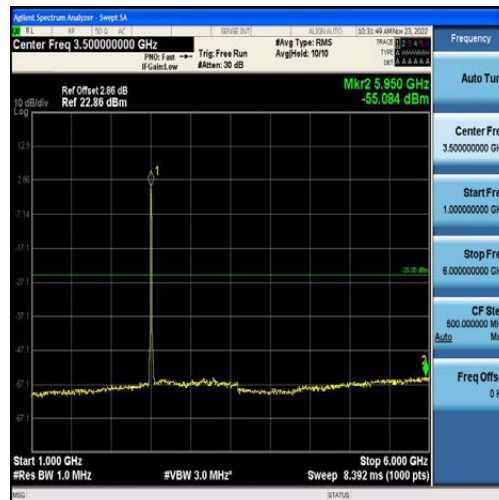
Band41-15MHz-QPSK-39725-75RB#0-Range2:1000~6000MHz
