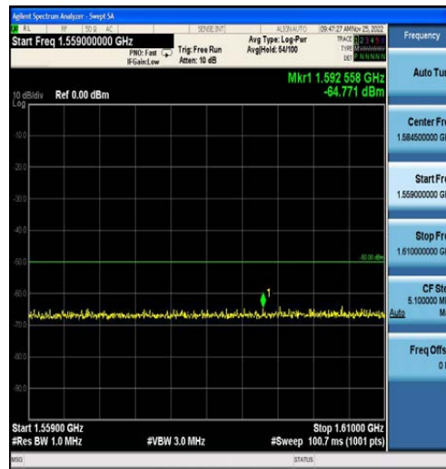
Band13-5MHz-16QAM-23205-25RB#0-Range3:1559~1610MHz
