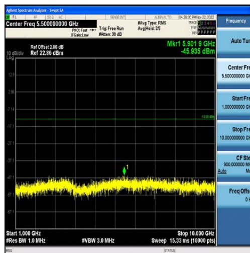
Band13-5MHz-16QAM-23205-25RB#0-Range2:1000~10000MHz
