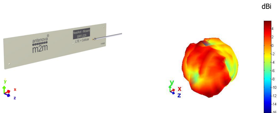
3D pattern at 2600 MHz Drag to rotate pattern and PCB by using Adobe Reader (Click to Activate)
