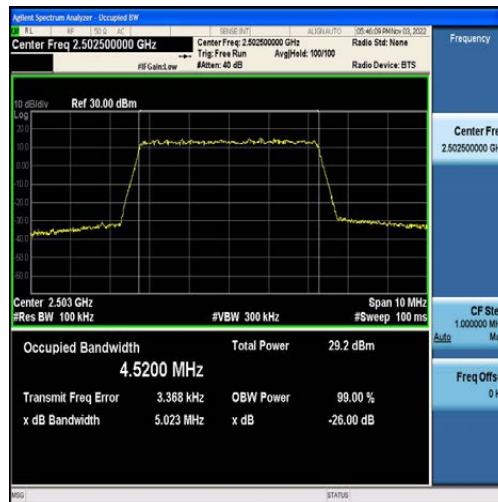
Band7-5MHz-QPSK-20775-25RB#0-4.5200
