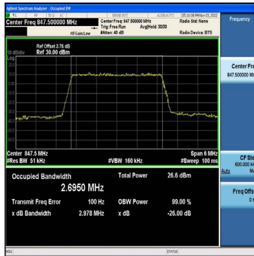
Band5-3MHz-16QAM-20635-15RB#0-2.6950
