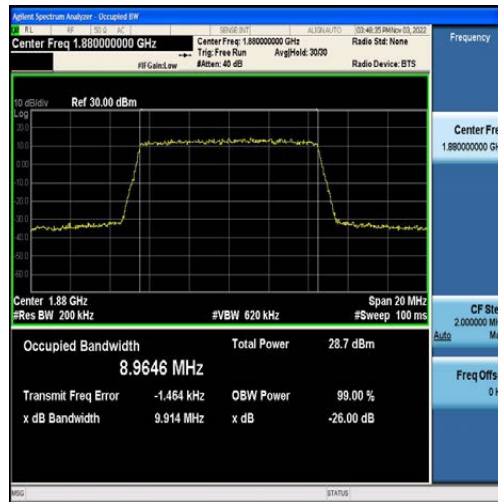
Band2-10MHz-QPSK-18900-50RB#0-8.9646
