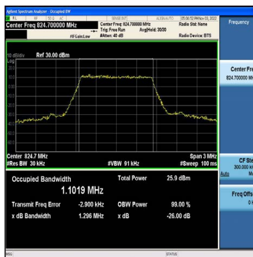
Band5-1.4MHz-16QAM-20407-6RB#0-1.1019
