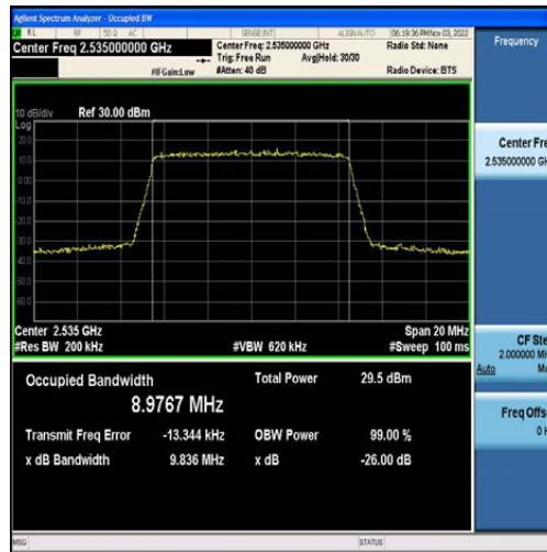
Band7-10MHz-QPSK-21100-50RB#0-8.9767
