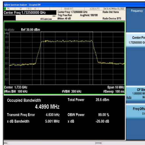
Band4-5MHz-QPSK-20175-25RB#0-4.4990
