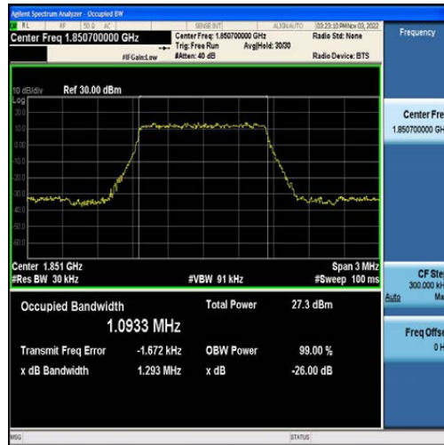
Band2-1.4MHz-QPSK-18607-6RB#0-1.0933
