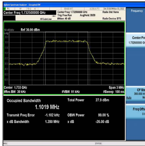
Band4-1.4MHz-QPSK-20175-6RB#0-1.1019
