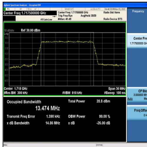
Band4-15MHz-QPSK-20025-75RB#0-13.474
