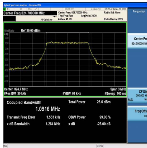
Band5-1.4MHz-QPSK-20407-6RB#0-1.0916
