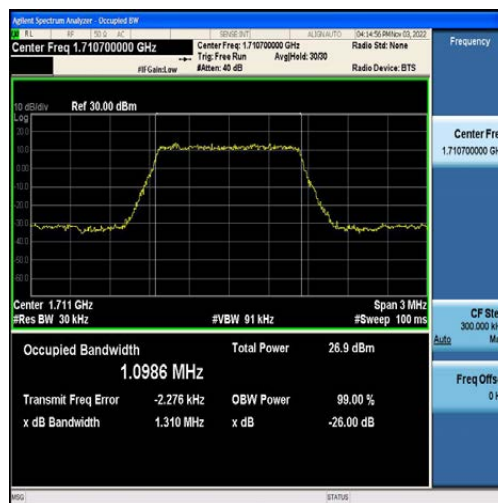
Band4-1.4MHz-16QAM-19957-6RB#0-1.0986
