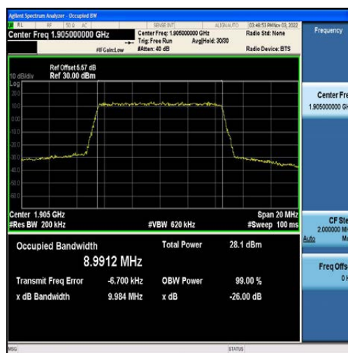
Band2-10MHz-QPSK-19150-50RB#0-8.9912
