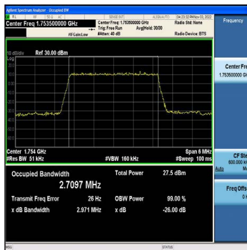
Band4-3MHz-QPSK-20385-15RB#0-2.7097
