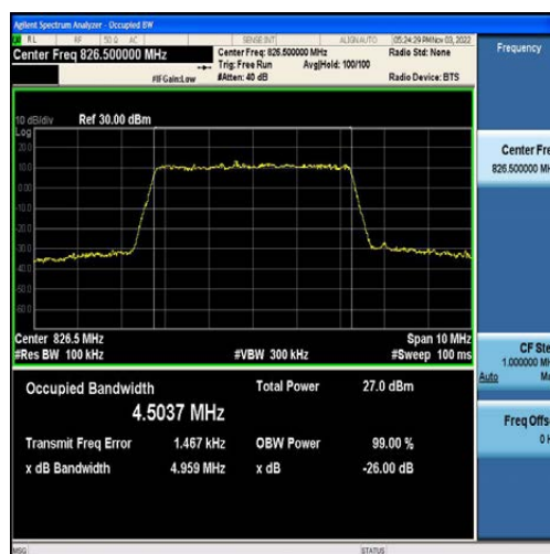
Band5-5MHz-16QAM-20425-25RB#0-4.5037
