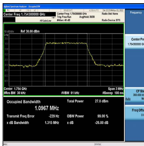
Band4-1.4MHz-QPSK-20393-6RB#0-1.0967
