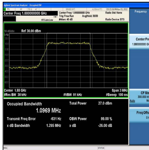
Band2-1.4MHz-16QAM-18900-6RB#0-1.0969
