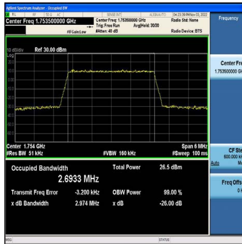
Band4-3MHz-16QAM-20385-15RB#0-2.6933
