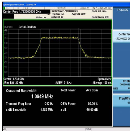
Band4-1.4MHz-16QAM-20175-6RB#0-1.0949
