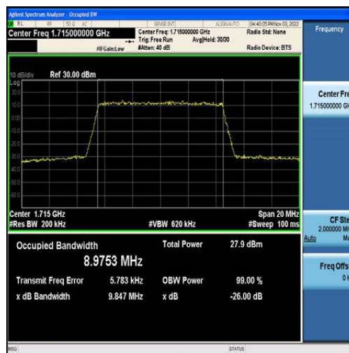
Band4-10MHz-16QAM-20000-50RB#0-8.9753
