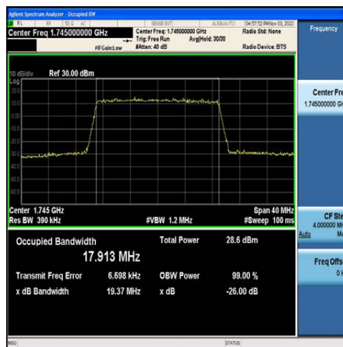
Band4-20MHz-QPSK-20300-100RB#0-17.913
