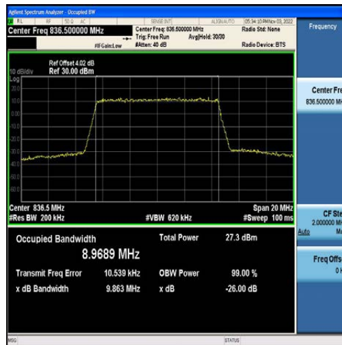
Band5-10MHz-16QAM-20525-50RB#0-8.9689
