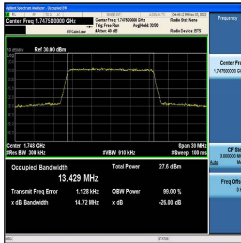
Band4-15MHz-16QAM-20325-75RB#0-13.429
