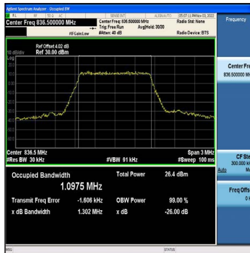
Band5-1.4MHz-16QAM-20525-6RB#0-1.0975
