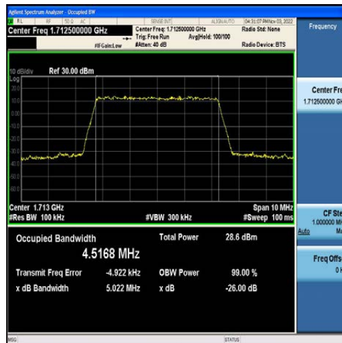
Band4-5MHz-QPSK-19975-25RB#0-4.5168
