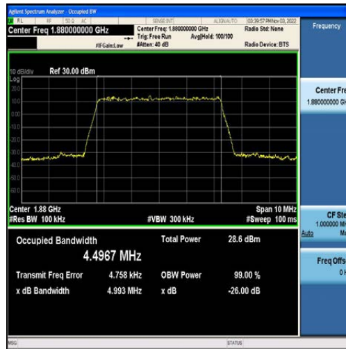
Band2-5MHz-QPSK-18900-25RB#0-4.4967
