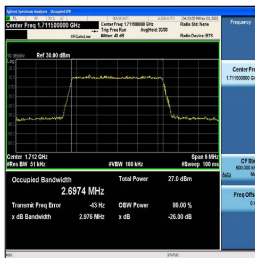
Band4-3MHz-16QAM-19965-15RB#0-2.6974
