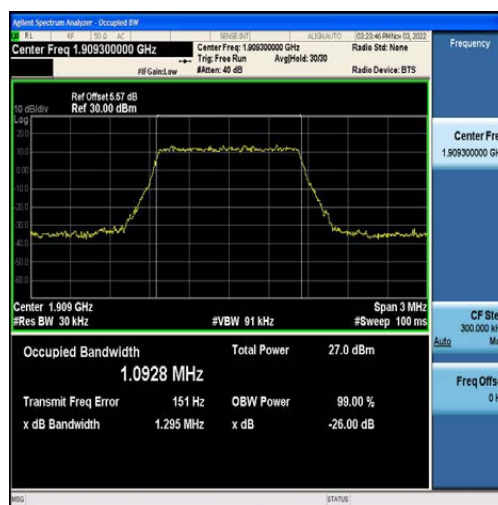
Band2-1.4MHz-QPSK-19193-6RB#0-1.0928
