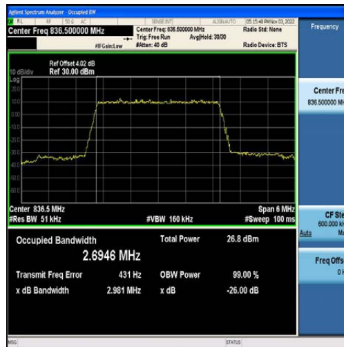
Band5-3MHz-16QAM-20525-15RB#0-2.6946
