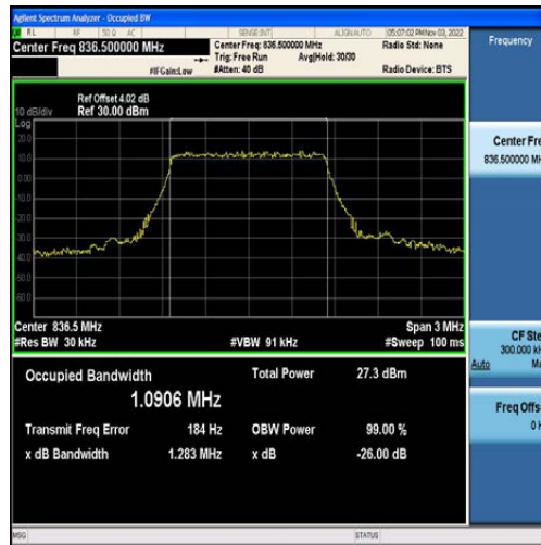
Band5-1.4MHz-QPSK-20525-6RB#0-1.0906
