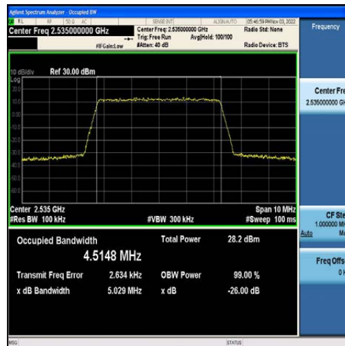
Band7-5MHz-16QAM-21100-25RB#0-4.5148
