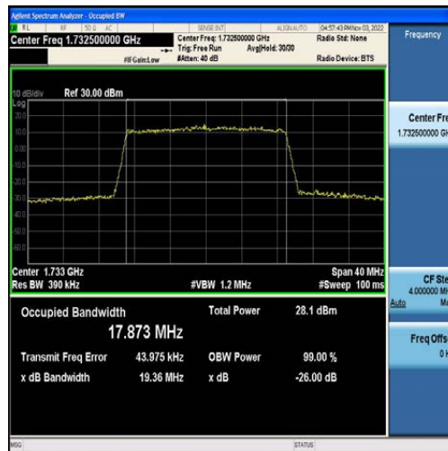
Band4-20MHz-16QAM-20175-100RB#0-17.873
