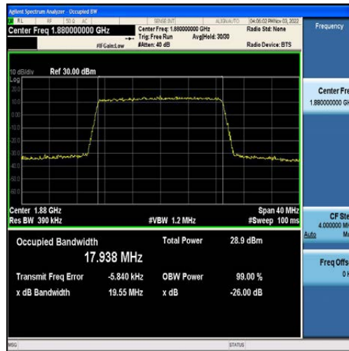
Band2-20MHz-QPSK-18900-100RB#0-17.938
