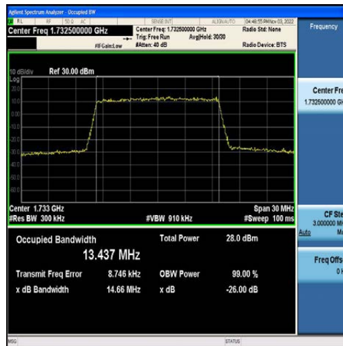
Band4-15MHz-16QAM-20175-75RB#0-13.437
