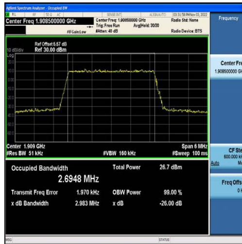
Band2-3MHz-16QAM-19185-15RB#0-2.6948
