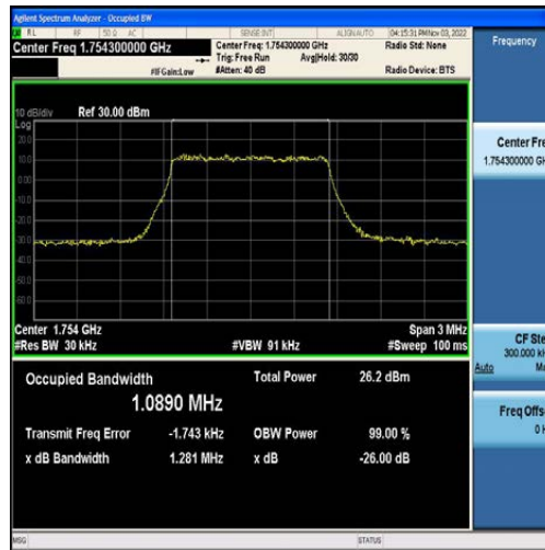
Band4-1.4MHz-16QAM-20393-6RB#0-1.0890
