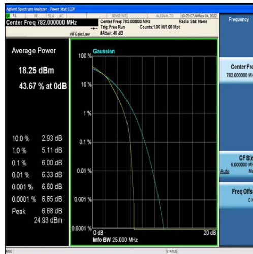
Band13-5MHz-16QAM-23230-25RB#0
