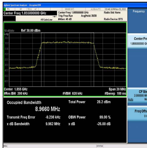
Band2-10MHz-QPSK-18650-50RB#0-8.9660
