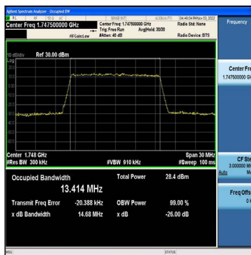
Band4-15MHz-QPSK-20325-75RB#0-13.414
