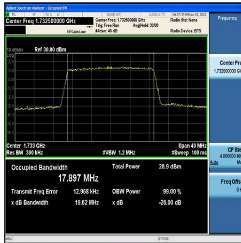
Band4-20MHz-QPSK-20175-100RB#0-17.897
