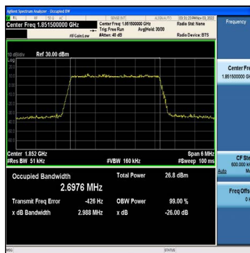
Band2-3MHz-16QAM-18615-15RB#0-2.6976
