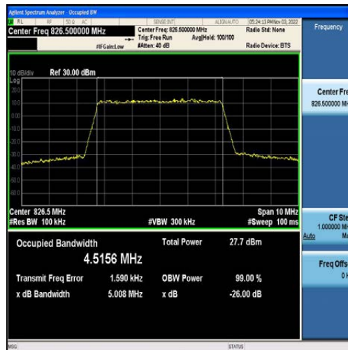
Band5-5MHz-QPSK-20425-25RB#0-4.5156
