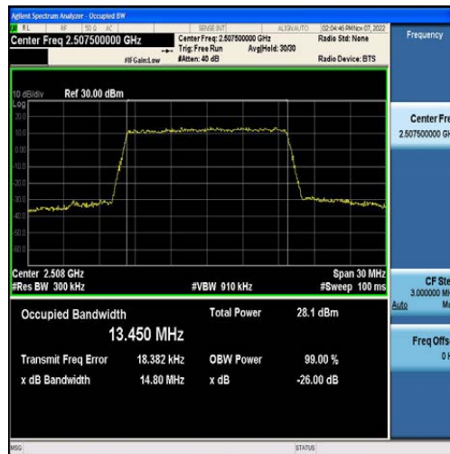
Band7-15MHz-QPSK-20825-75RB#0-13.450
