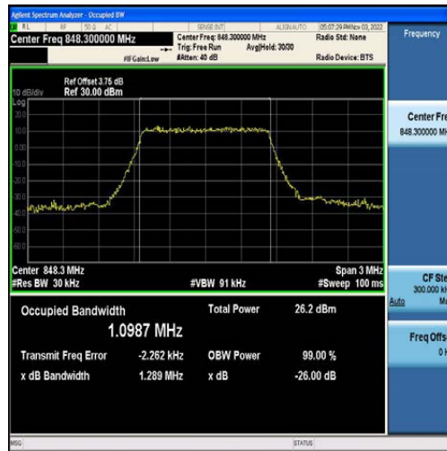
Band5-1.4MHz-16QAM-20643-6RB#0-1.0987
