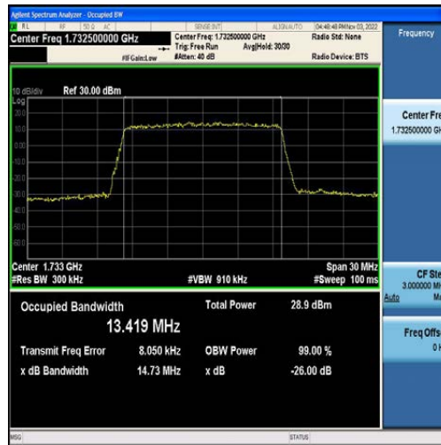
Band4-15MHz-QPSK-20175-75RB#0-13.419
