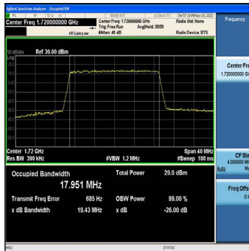
Band4-20MHz-QPSK-20050-100RB#0-17.951
