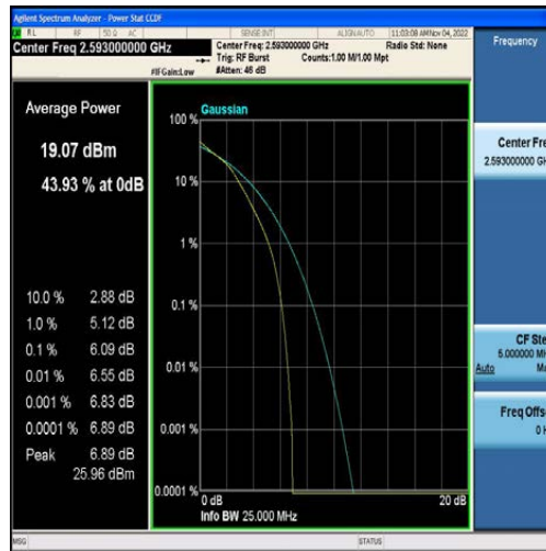
Band41-10MHz-16QAM-40620-50RB#0
