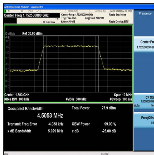
Band4-5MHz-QPSK-20375-25RB#0-4.5053
