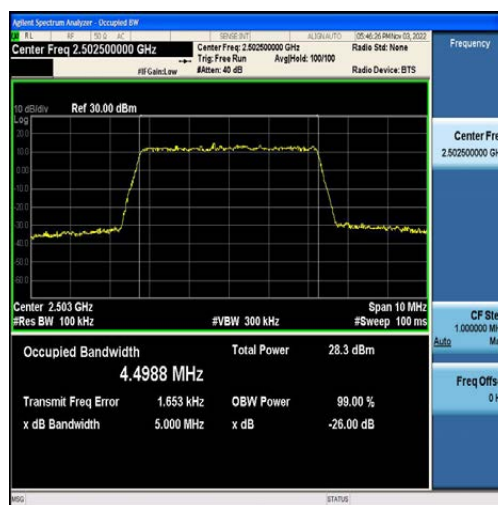
Band7-5MHz-16QAM-20775-25RB#0-4.4988
