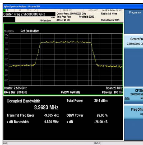
Band7-10MHz-QPSK-21400-50RB#0-8.9683
