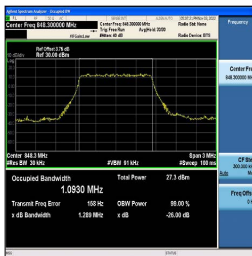
Band5-1.4MHz-QPSK-20643-6RB#0-1.0930
