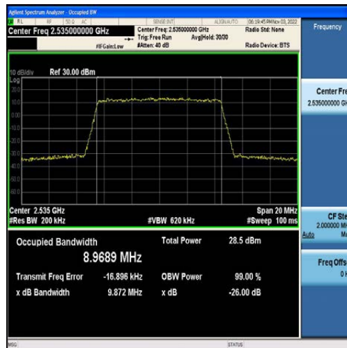
Band7-10MHz-16QAM-21100-50RB#0-8.9689
