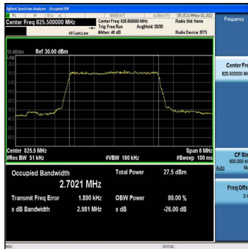
Band5-3MHz-QPSK-20415-15RB#0-2.7021
