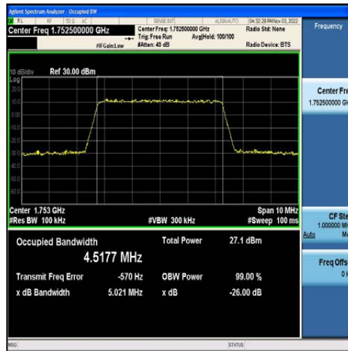
Band4-5MHz-16QAM-20375-25RB#0-4.5177
