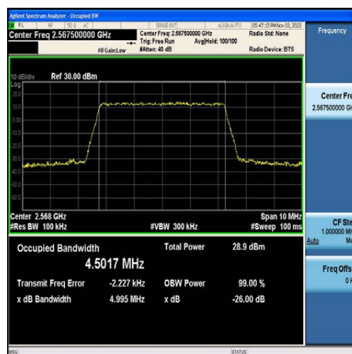
Band7-5MHz-QPSK-21425-25RB#0-4.5017
