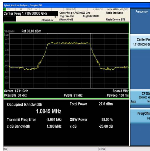
Band4-1.4MHz-QPSK-19957-6RB#0-1.0949
