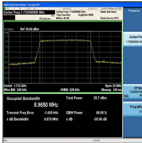
Band4-10MHz-QPSK-20175-50RB#0-8.9650
