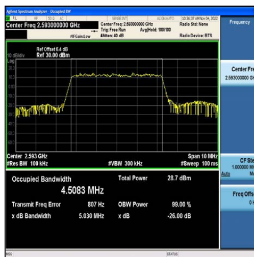
Band41-5MHz-QPSK-40620-25RB#0-4.5083
