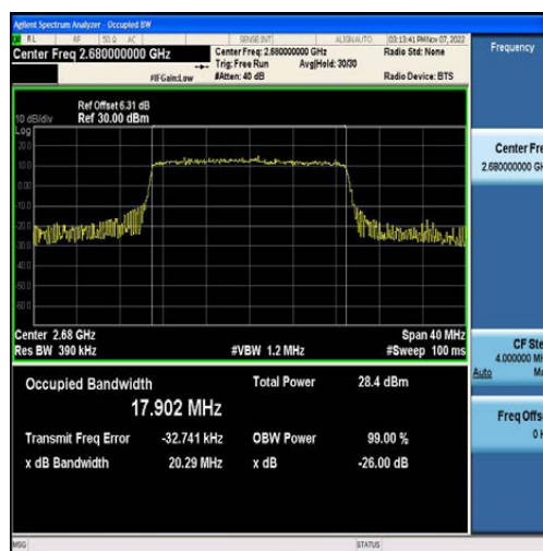
Band41-20MHz-16QAM-41490-100RB#0-17.902
