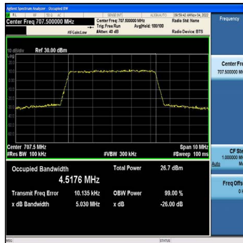
Band12-5MHz-16QAM-23095-25RB#0-4.5176
