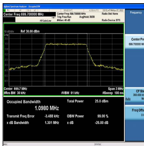
Band12-1.4MHz-16QAM-23017-6RB#0-1.0980
