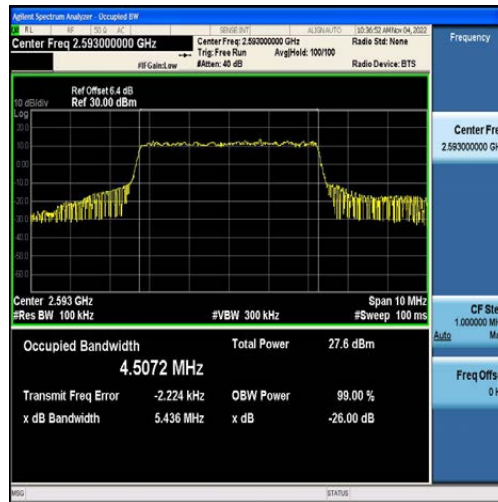
Band41-5MHz-16QAM-40620-25RB#0-4.5072
