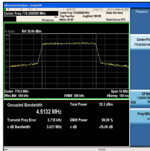
Band13-5MHz-QPSK-23205-25RB#0-4.5132
