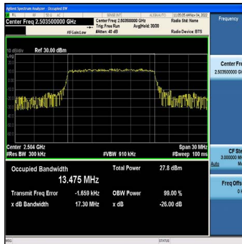
Band41-15MHz-16QAM-39725-75RB#0-13.475
