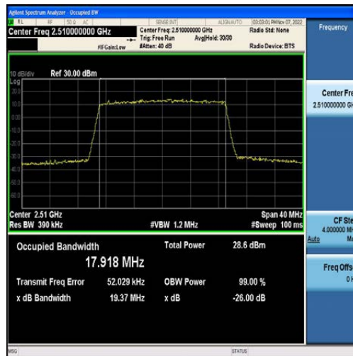
Band7-20MHz-16QAM-20850-100RB#0-17.918
