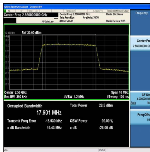
Band7-20MHz-16QAM-21350-100RB#0-17.901
