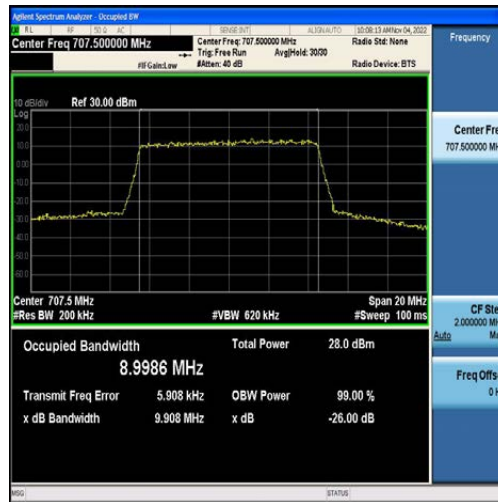
Band12-10MHz-QPSK-23095-50RB#0-8.9986
