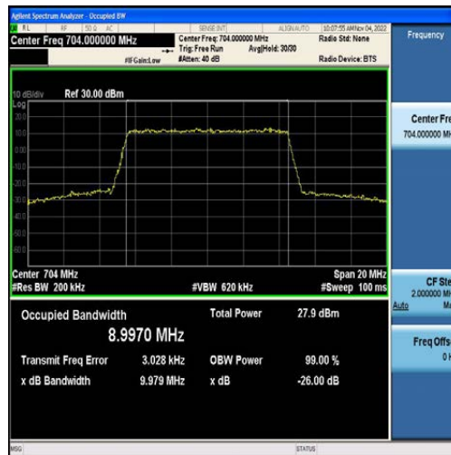
Band12-10MHz-QPSK-23060-50RB#0-8.9970
