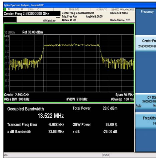
Band41-15MHz-16QAM-40620-75RB#0-13.522
