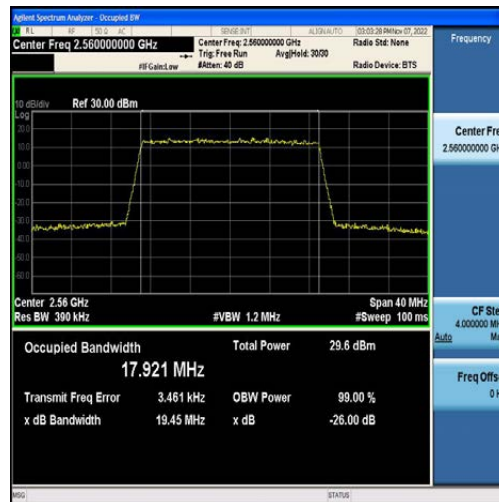
Band7-20MHz-QPSK-21350-100RB#0-17.921
