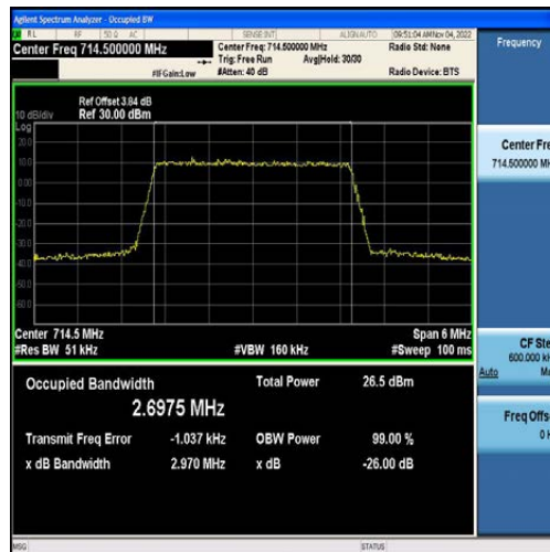
Band12-3MHz-16QAM-23165-15RB#0-2.6975
