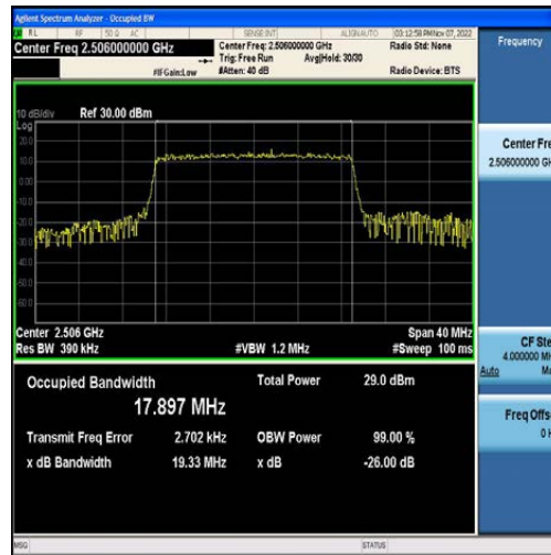
Band41-20MHz-QPSK-39750-100RB#0-17.897
