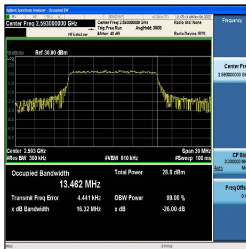
Band41-15MHz-QPSK-40620-75RB#0-13.462
