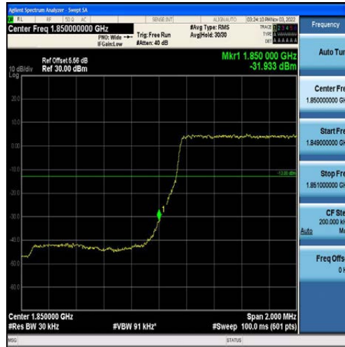
Band2-1.4MHz-QPSK-18607-6RB#0
