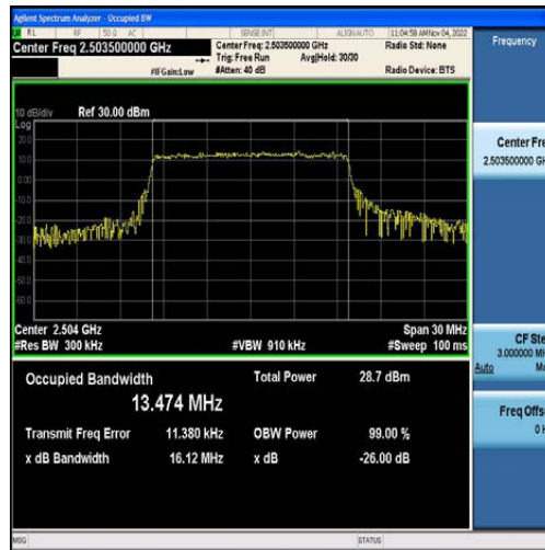
Band41-15MHz-QPSK-39725-75RB#0-13.474
