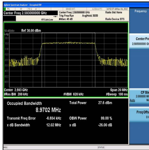
Band41-10MHz-16QAM-40620-50RB#0-8.9702
