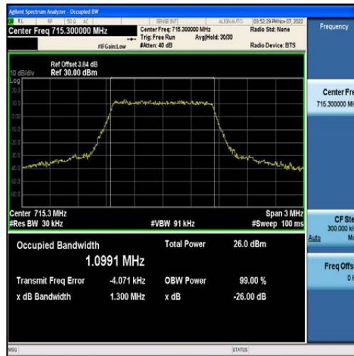
Band12-1.4MHz-16QAM-23173-6RB#0-1.0991
