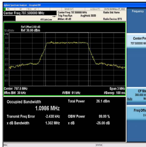
Band12-1.4MHz-16QAM-23095-6RB#0-1.0986
