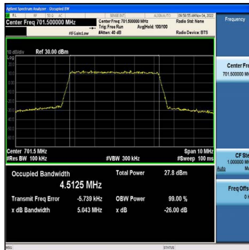
Band12-5MHz-QPSK-23035-25RB#0-4.5125
