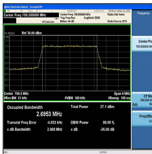
Band12-3MHz-QPSK-23025-15RB#0-2.6953
