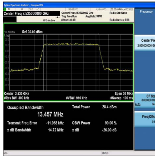
Band7-15MHz-QPSK-21100-75RB#0-13.457
