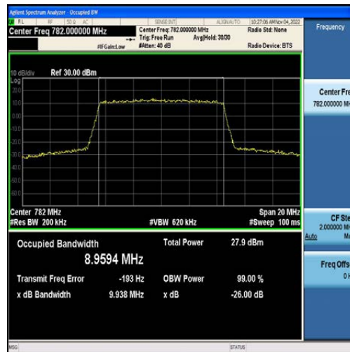
Band13-10MHz-QPSK-23230-50RB#0-8.9594
