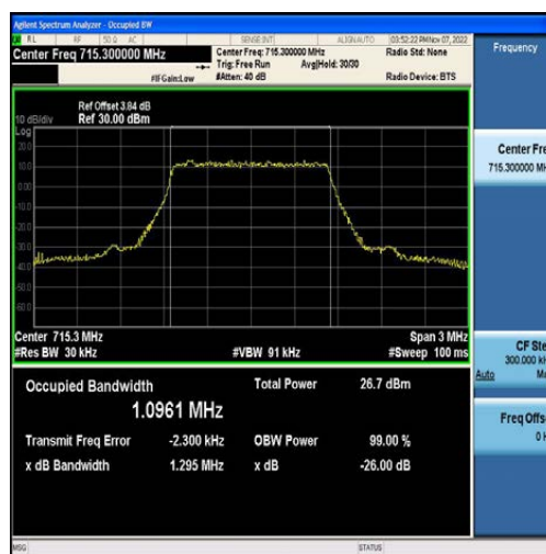
Band12-1.4MHz-QPSK-23173-6RB#0-1.0961
