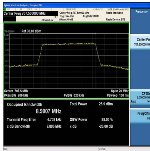
Band12-10MHz-16QAM-23095-50RB#0-8.9907
