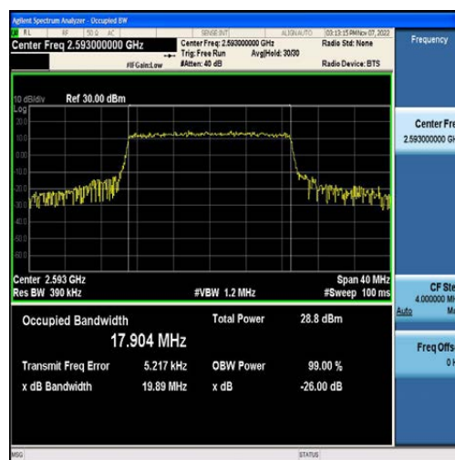
Band41-20MHz-QPSK-40620-100RB#0-17.904
