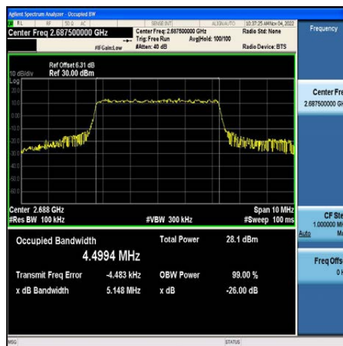
Band41-5MHz-16QAM-41565-25RB#0-4.4994
