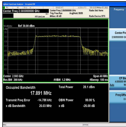
Band41-20MHz-16QAM-40620-100RB#0-17.891
