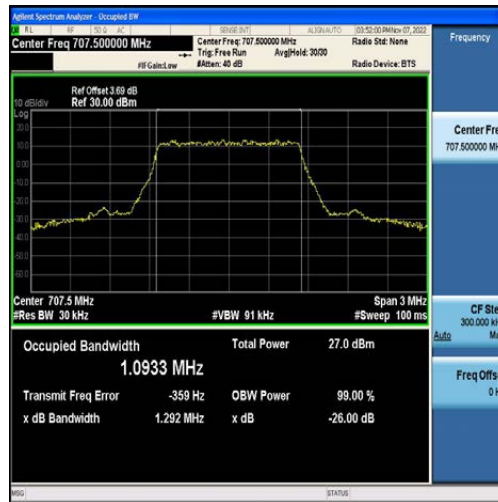
Band12-1.4MHz-QPSK-23095-6RB#0-1.0933
