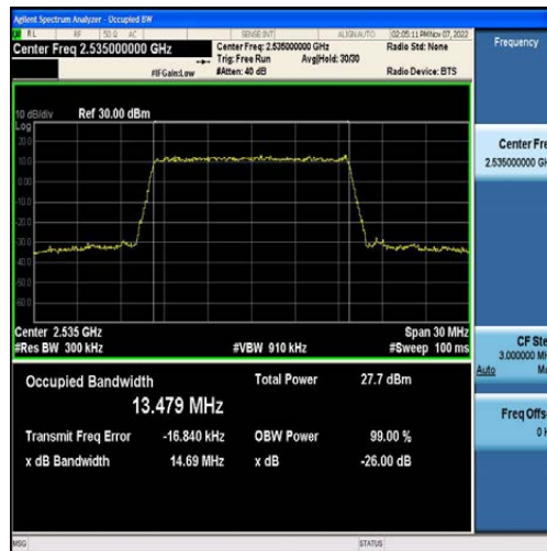
Band7-15MHz-16QAM-21100-75RB#0-13.479
