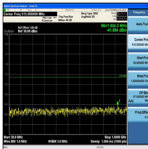
Band2-5MHz-QPSK-18625-25RB#0-Range1:30~1000MHz
