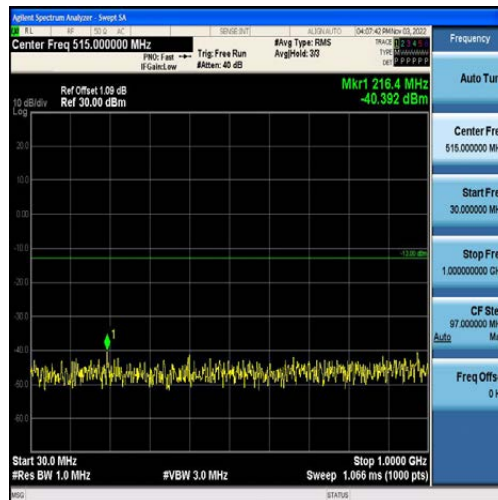
Band2-20MHz-16QAM-18700-100RB#0-Range1:30~1000MHz
