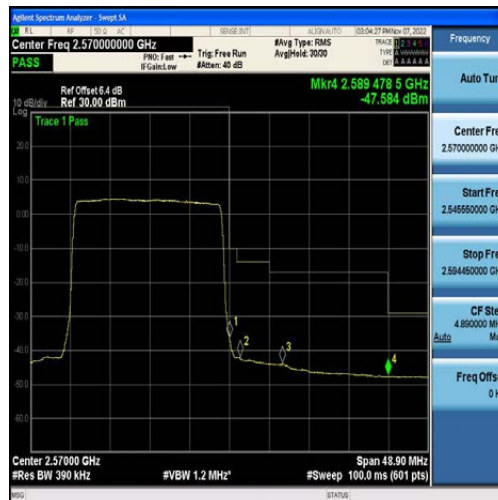
Band7-20MHz-QPSK-21350-100RB#0
