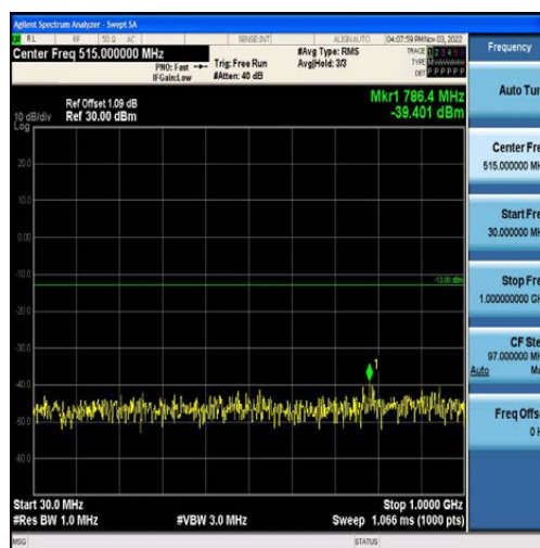
Band2-20MHz-16QAM-18900-100RB#0-Range1:30~1000MHz
