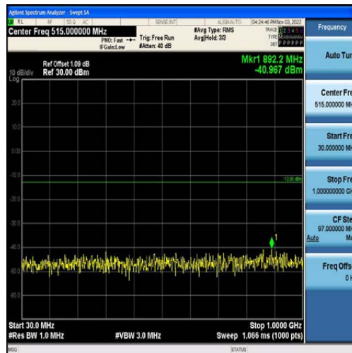
Band4-3MHz-16QAM-19965-15RB#0-Range1:30~1000MHz
