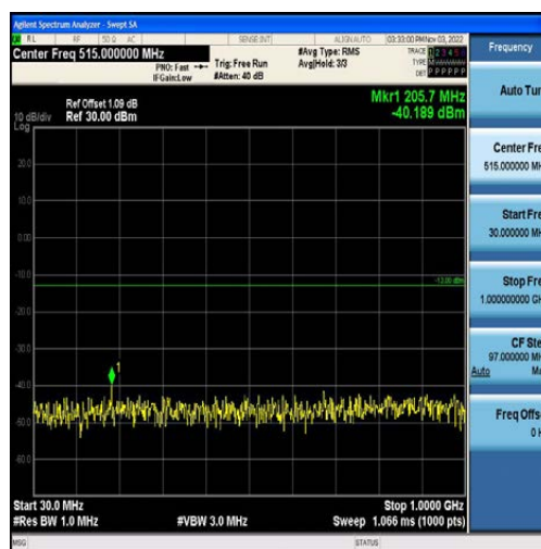
Band2-3MHz-QPSK-18615-15RB#0-Range1:30~1000MHz
