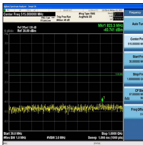
Band2-15MHz-QPSK-18675-75RB#0-Range1:30~1000MHz
