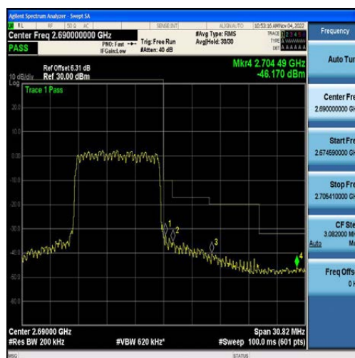
Band41-10MHz-QPSK-41540-50RB#0
