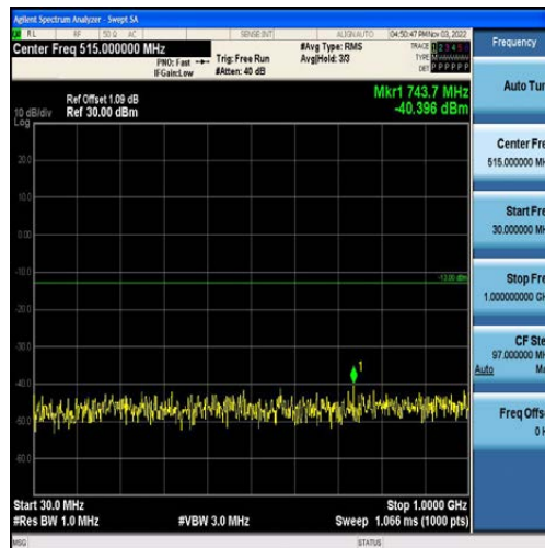
Band4-15MHz-QPSK-20325-75RB#0-Range1:30~1000MHz
