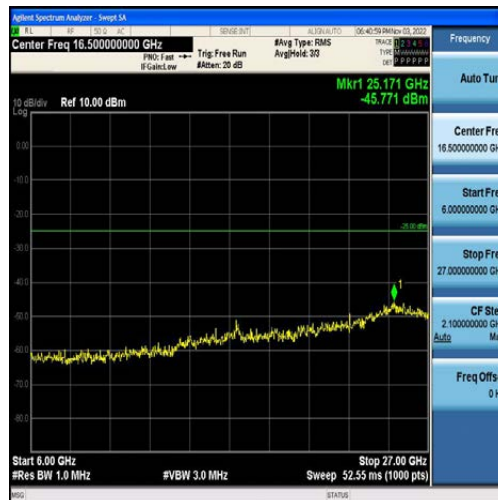
Band7-15MHz-QPSK-21375-75RB#0-Range3:6000~27000MHz
