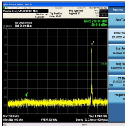
Band5-5MHz-QPSK-20625-25RB#0-Range1:30~1000MHz
