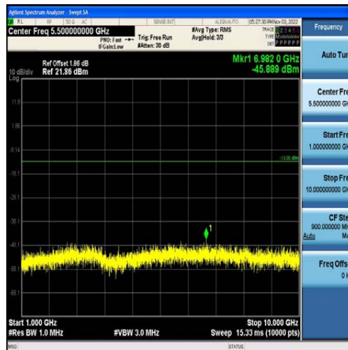
Band5-5MHz-16QAM-20625-25RB#0-Range2:1000~10000MHz
