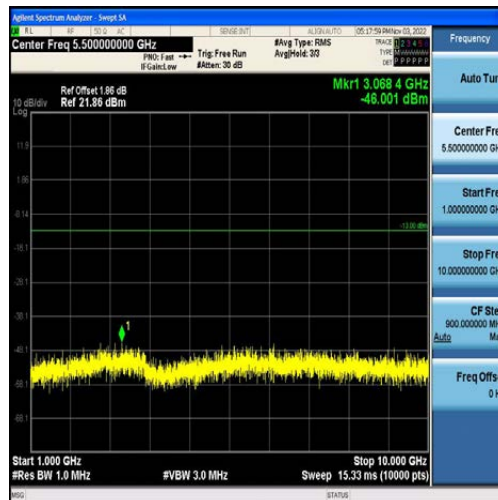
Band5-3MHz-16QAM-20635-15RB#0-Range2:1000~10000MHz
