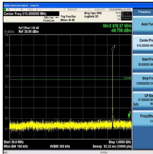
Band5-1.4MHz-QPSK-20643-6RB#0-Range1:30~1000MHz
