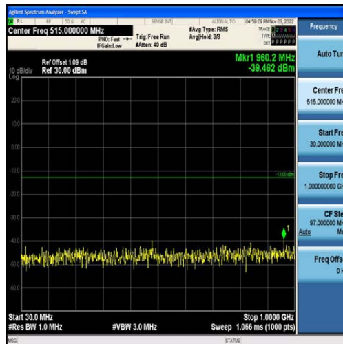
Band4-20MHz-16QAM-20050-100RB#0-Range1:30~1000MHz
