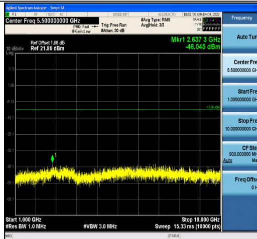
Band12-5MHz-QPSK-23155-25RB#0-Range2:1000~10000MHz
