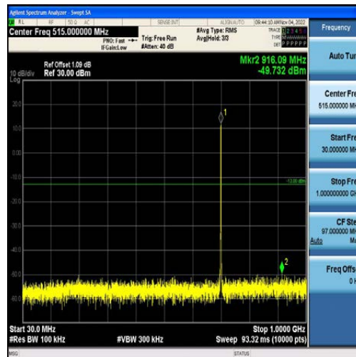
Band12-1.4MHz-16QAM-23095-6RB#0-Range1:30~1000MHz
