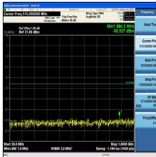
Band41-10MHz-QPSK-40620-50RB#0-Range1:30~1000MHz
