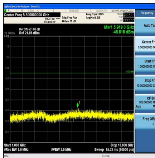
Band13-5MHz-16QAM-23205-25RB#0-Range2:1000~10000MHz
