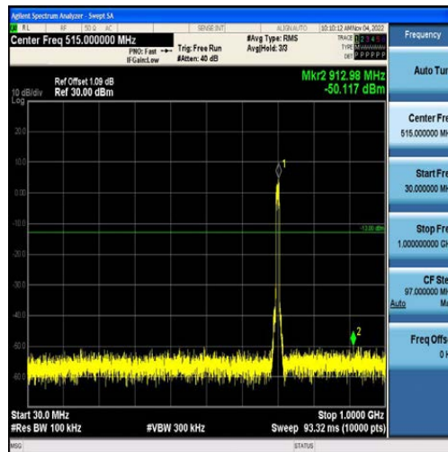
Band12-10MHz-16QAM-23095-50RB#0-Range1:30~1000MHz
