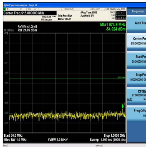
Band41-15MHz-16QAM-39725-75RB#0-Range1:30~1000MHz
