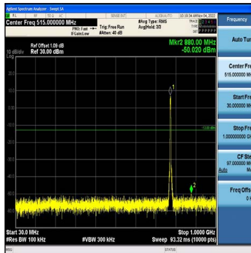
Band13-5MHz-QPSK-23205-25RB#0-Range1:30~1000MHz
