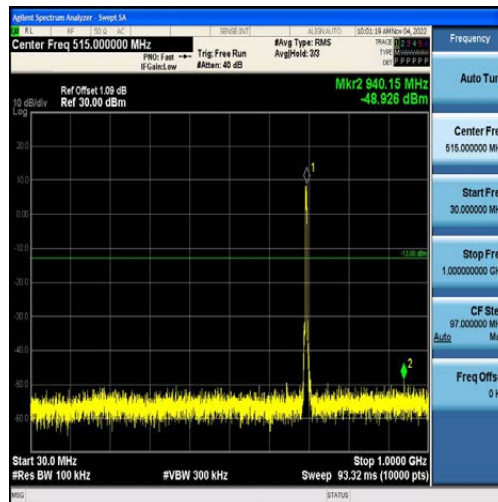
Band12-5MHz-QPSK-23035-25RB#0-Range1:30~1000MHz
