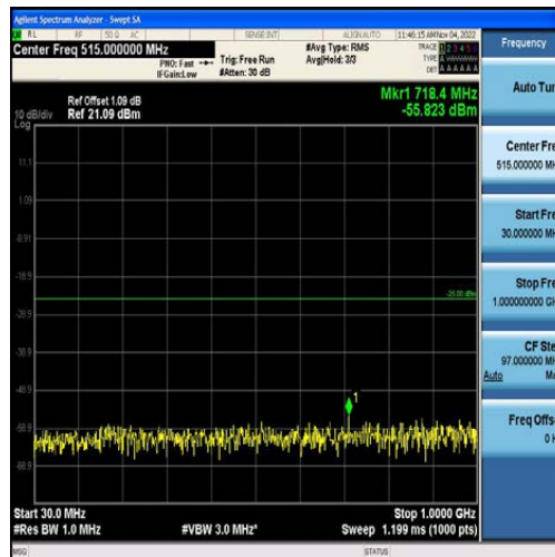
Band41-15MHz-16QAM-40620-75RB#0-Range1:30~1000MHz
