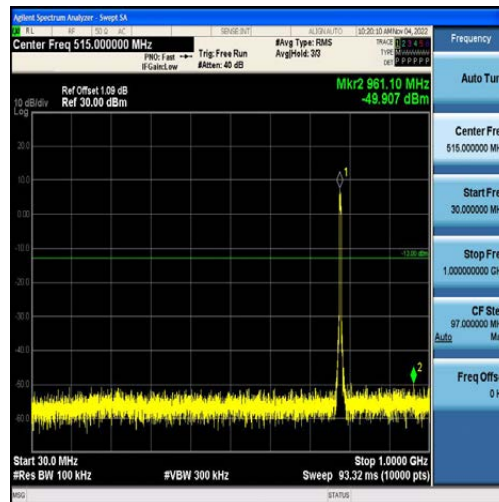
Band13-5MHz-16QAM-23230-25RB#0-Range1:30~1000MHz
