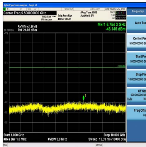
Band12-10MHz-16QAM-23060-50RB#0-Range2:1000~10000MHz
