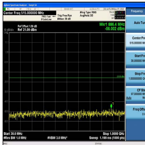
Band41-20MHz-QPSK-39750-100RB#0-Range1:30~1000MHz
