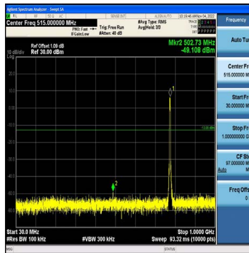
Band13-5MHz-16QAM-23205-25RB#0-Range1:30~1000MHz
