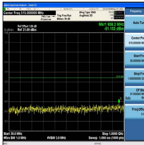
Band7-20MHz-16QAM-20850-100RB#0-Range1:30~1000MHz
