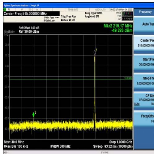
Band12-3MHz-QPSK-23025-15RB#0-Range1:30~1000MHz
