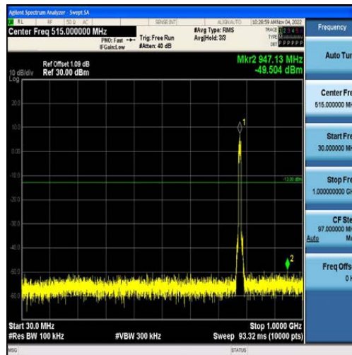
Band13-10MHz-QPSK-23230-50RB#0-Range1:30~1000MHz
