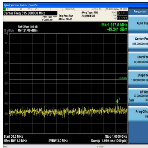
Band7-20MHz-16QAM-21100-100RB#0-Range1:30~1000MHz
