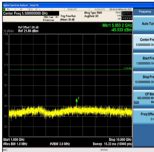
Band12-1.4MHz-QPSK-23173-6RB#0-Range2:1000~10000MHz
