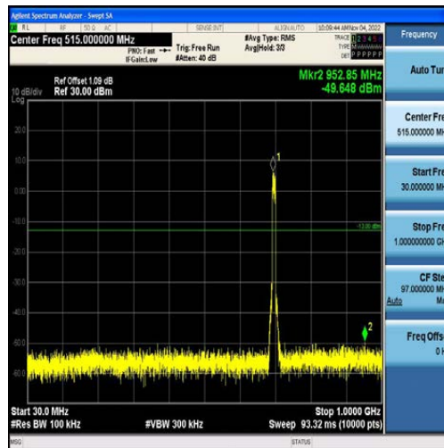
Band12-10MHz-QPSK-23060-50RB#0-Range1:30~1000MHz
