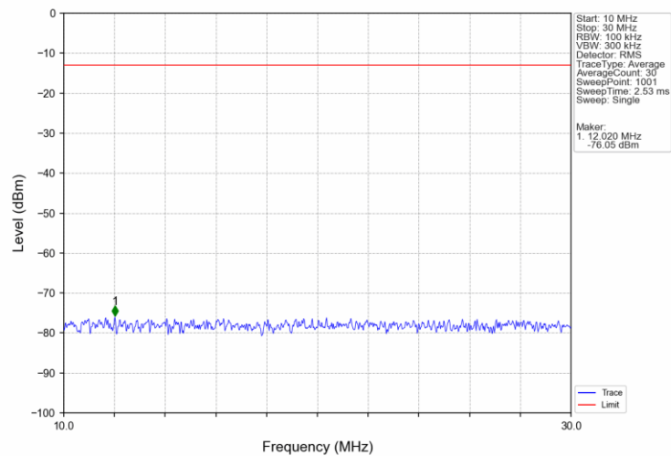
Band12 3MHz QPSK LCH 700.5MHz RB 1 0 NTN
