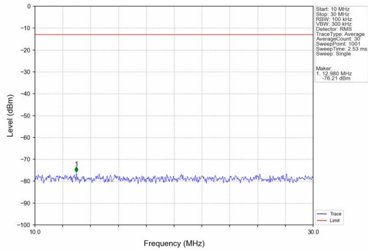
Band12 1.4MHz 16QAM LCH 699.7MHz RB 1 0 NTNV
