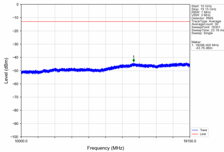
Band25_10MHz_16QAM_HCH_1910MHz_RB_1_0_NTNV
