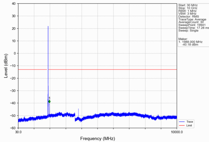
Band25_10MHz_16QAM_HCH_1910MHz_RB_1_0_NTNV
