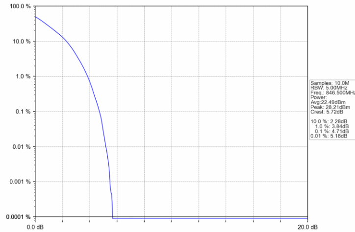
Band26b 5MHz QPSK HCH 846.5MHz RB 25 0 NTN
