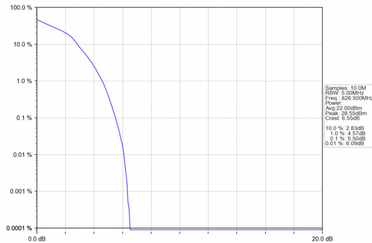
Band26b 5MHz 16QAM LCH 826.5MHz RB 25 0 NTN
