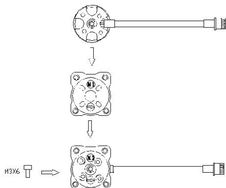
M1 Install Motor inclined mount
