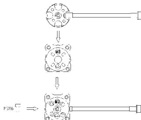
M2 Install Motor inclined mount
