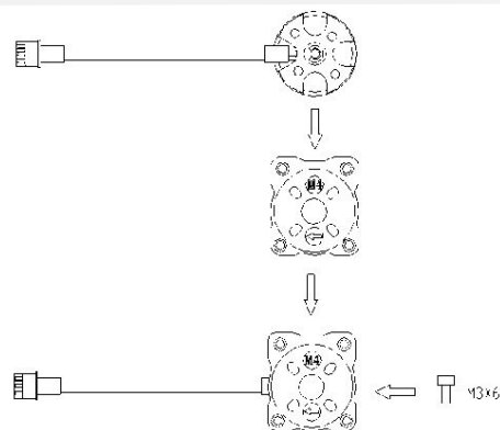
M4 Install Motor inclined mout
