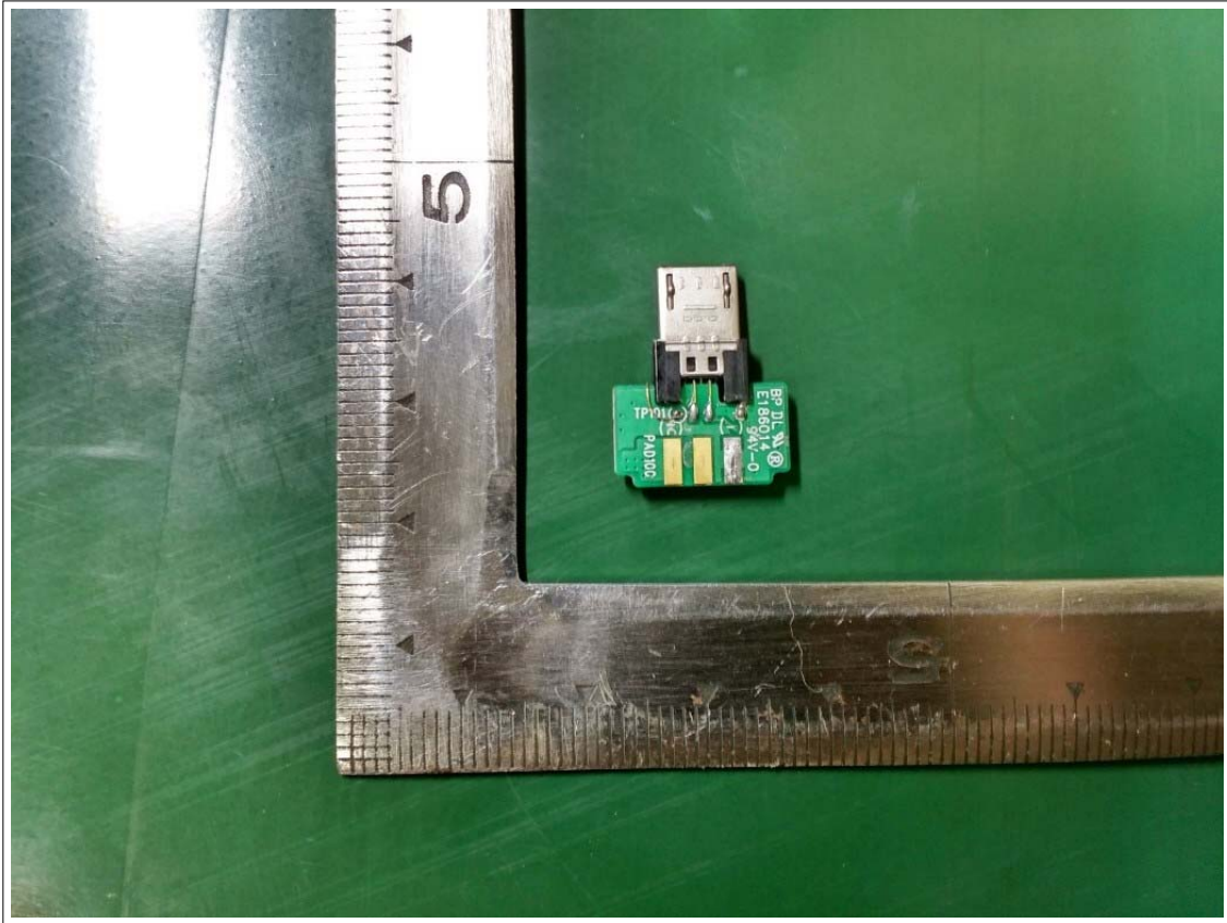
View of Mobile phone Charge PCB(Top)
