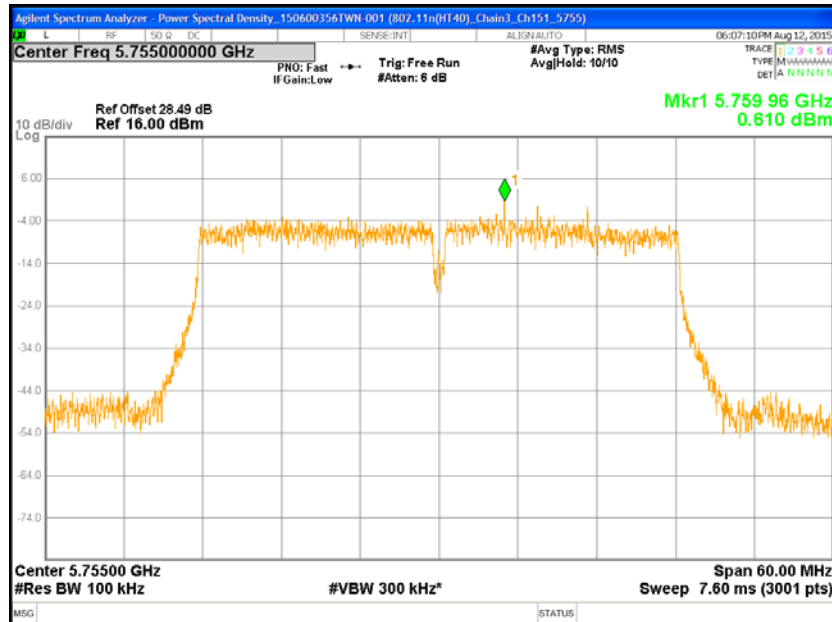
Chain3 : Power Spectral Density @ 802.11an(HT40) Mode Ch151
