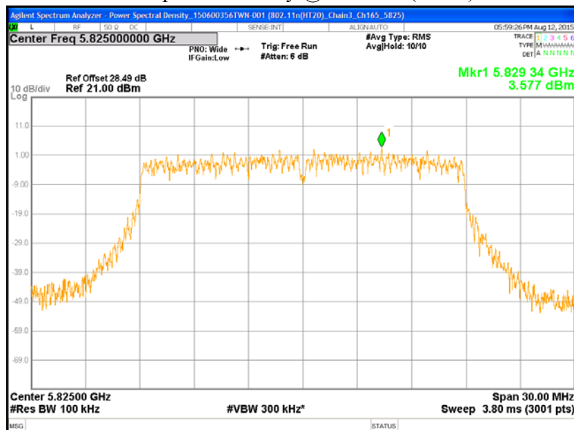
Chain3 : Power Spectral Density @ 802.11an(HT20) Mode Ch165
