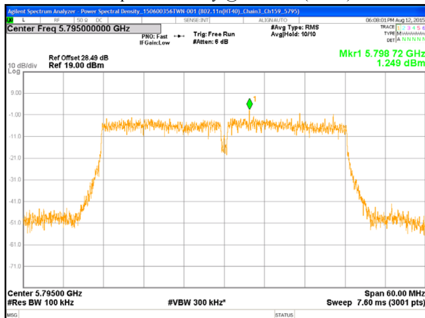
Chain3 : Power Spectral Density @ 802.11an(HT40) Mode Ch159
