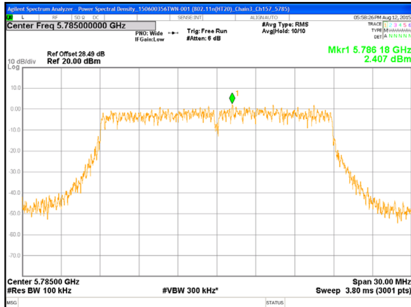
Chain3 : Power Spectral Density @ 802.11an(HT20) Mode Ch157
