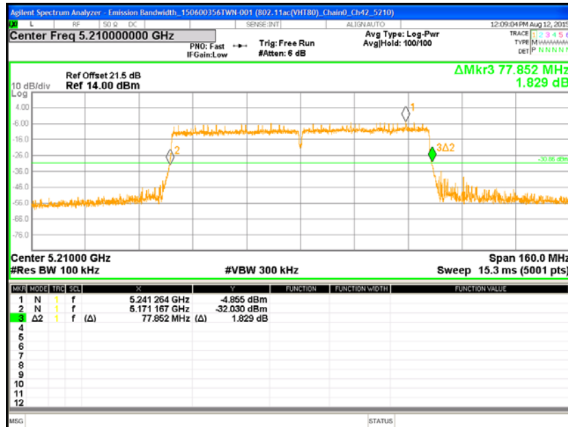
Chain0 : 26dB Bandwidth @ 802.11ac(VHT80) mode Ch42
