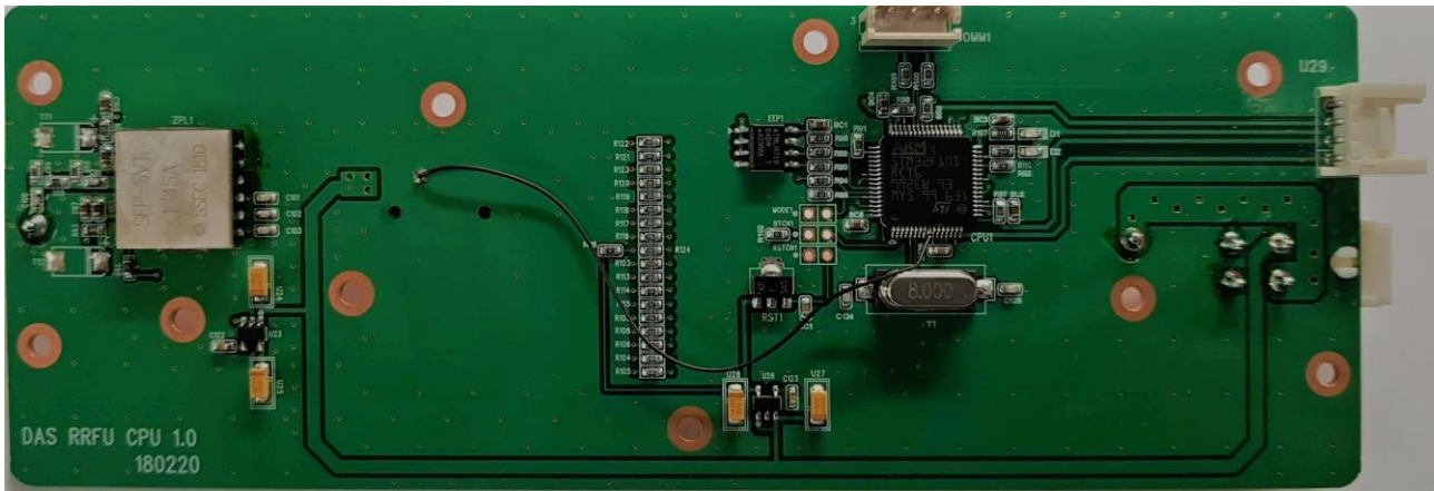
_PCB Top_MCU
