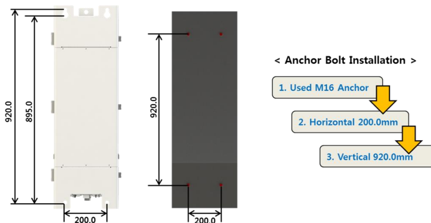
Figure 8. ROU 5W Anchor Bolt Assemble.
