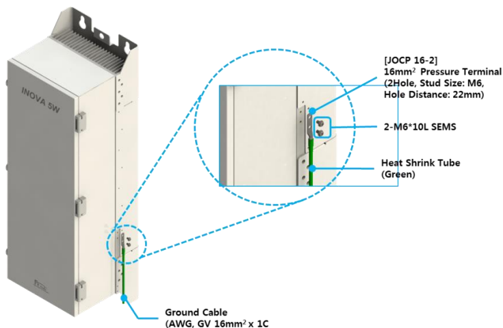
Figure 10. ROU 5W Ground Cable Connection.
