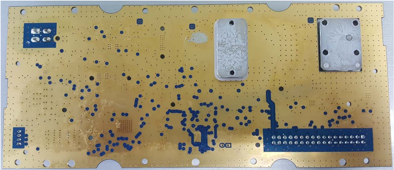
_PCB Bottom_TX
