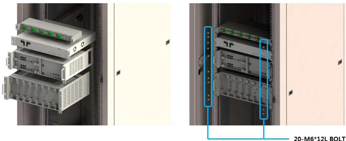
Figure 15. Within 19" Rack, MHU installation.
