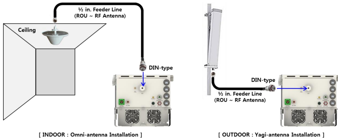
Figure 31. ROU 5W Antenna and Cable Connection.
