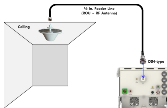
Figure 24. ROU 2W Antenna and Cable Connection.
