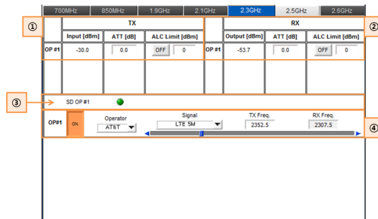
Figure 49. 2.3GHz MHU Band Information Screen.
