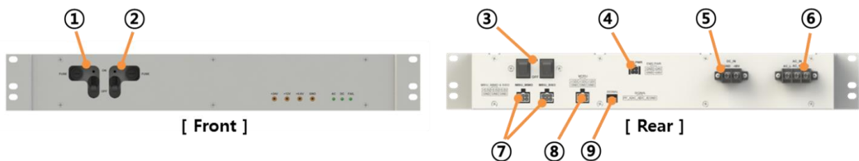
Figure 6. MPSU Port Configuration.
