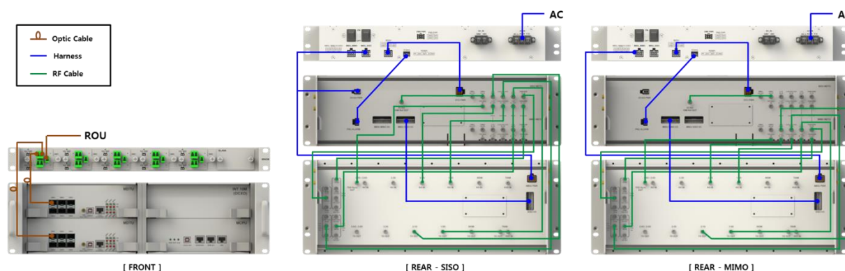
Figure 16. MHU Cable Connection.
