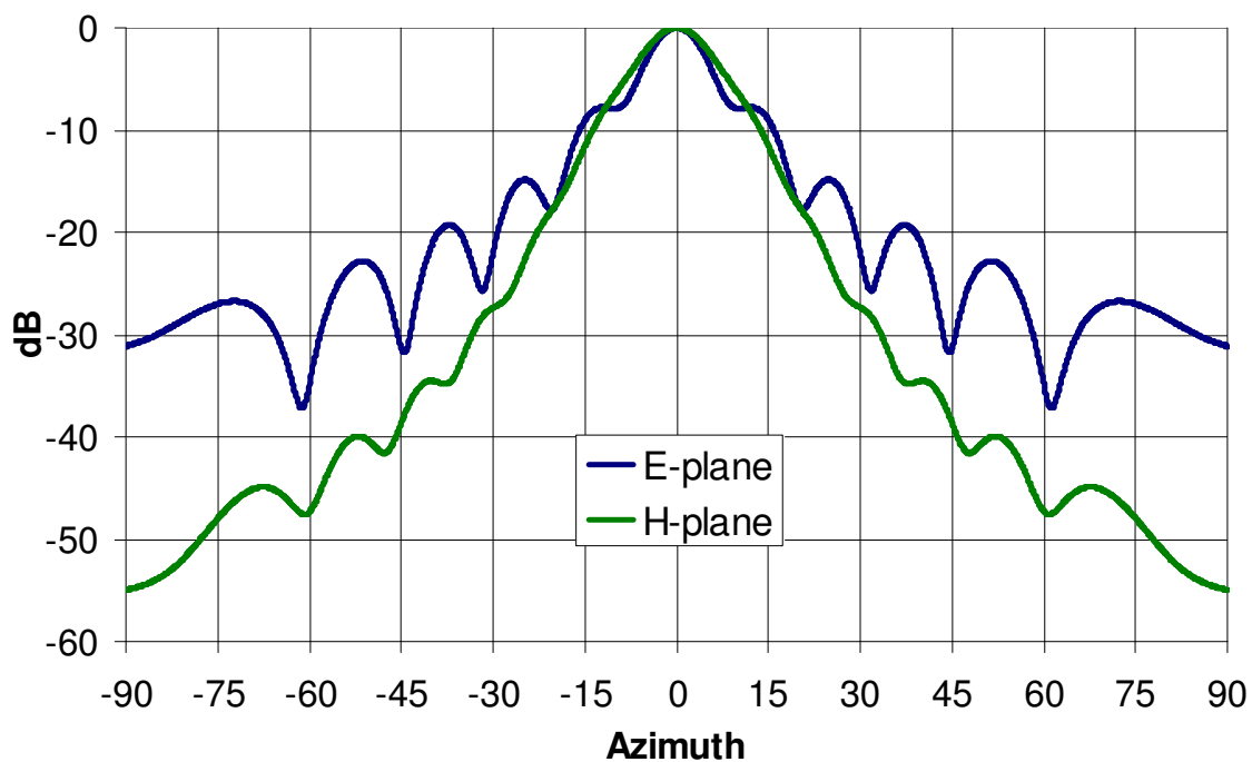
HO6 Radiation Pattern @ 140 GHz
