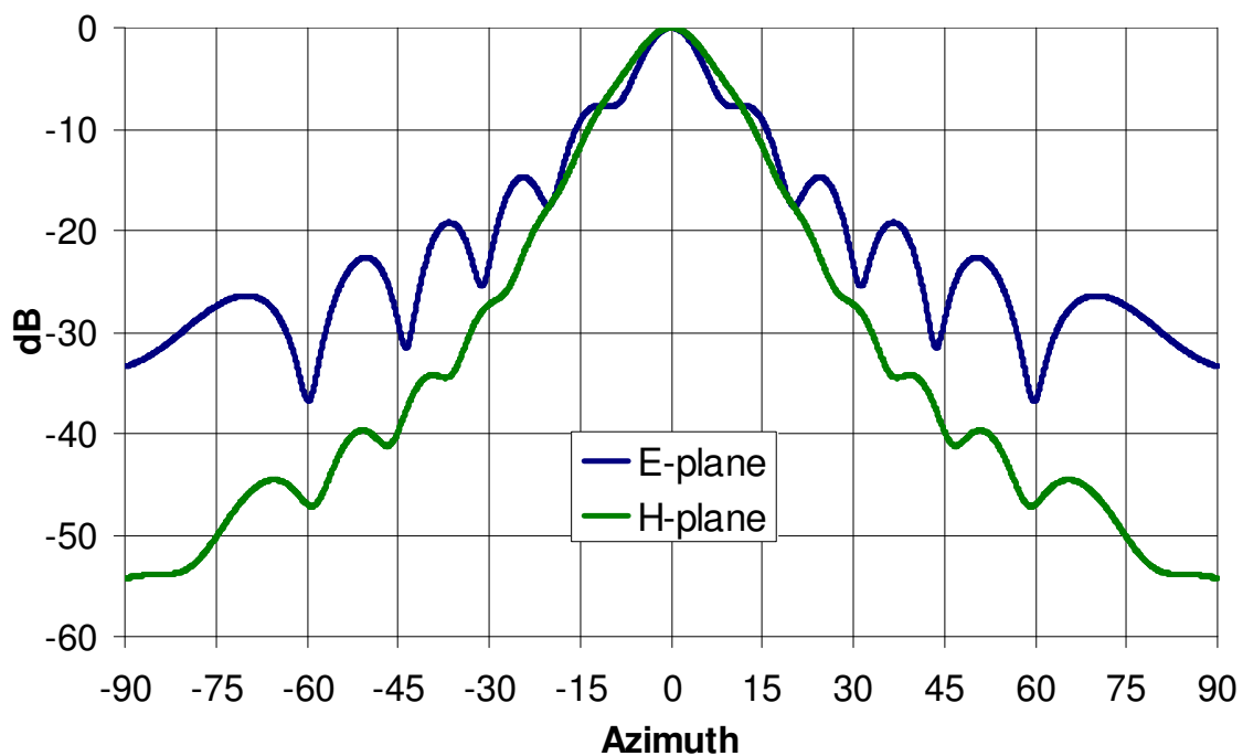
HO4 Radiation Pattern @ 215 GHz
