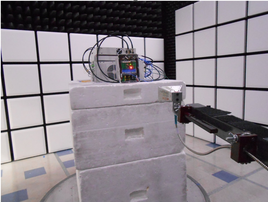
Radiated RF_40 - 50 GHz
