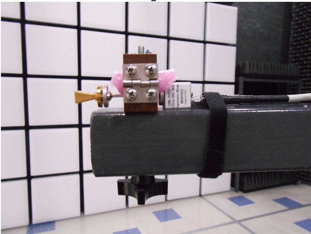
Radiated RF_170 - 200 GHz
