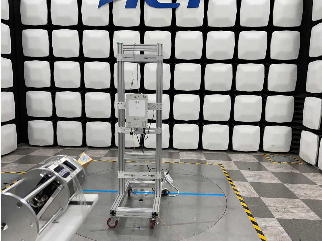
Radiated Test Setup Photo – Spurious (WR-19 Horn Antenna, 135°)
