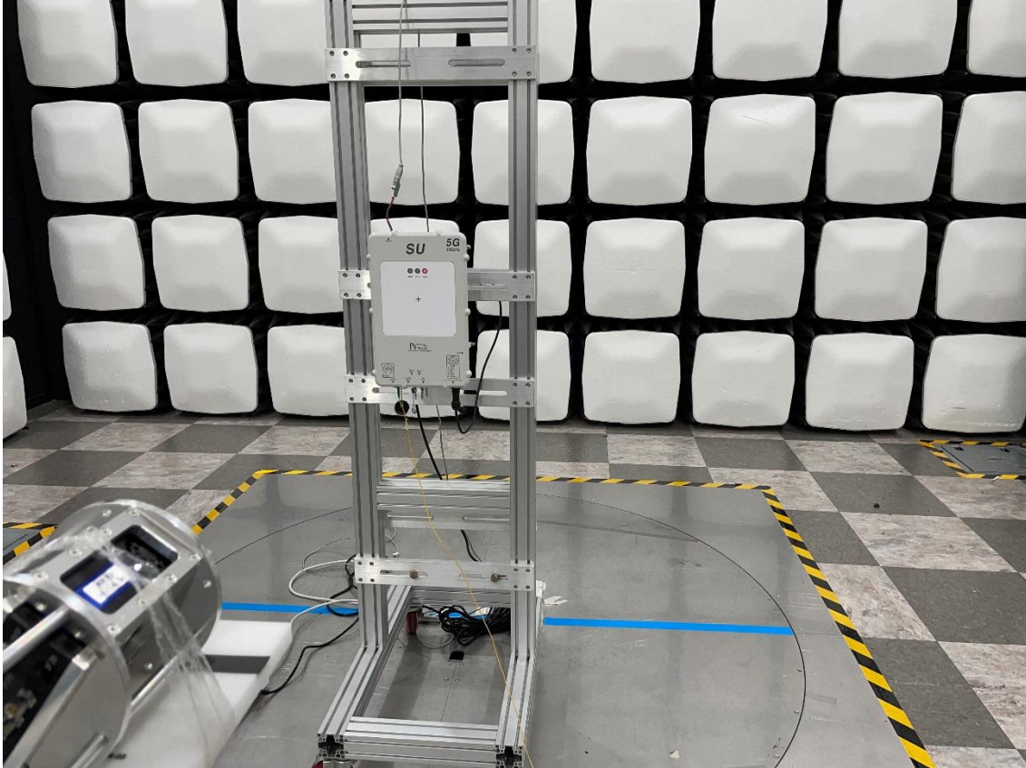
Radiated Test Setup Photo – Spurious (WR-08 Horn Antenna, 135°)
