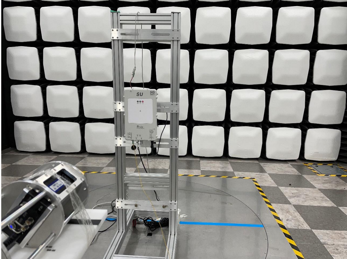
Radiated Test Setup Photo – Spurious (WR-12 Horn Antenna, 45°)
