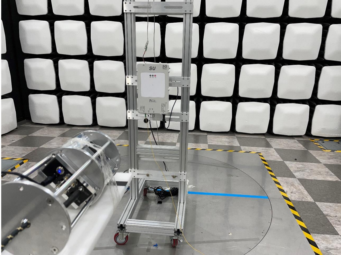
Radiated Test Setup Photo – Spurious (WR-12 Horn Antenna, 135°)
