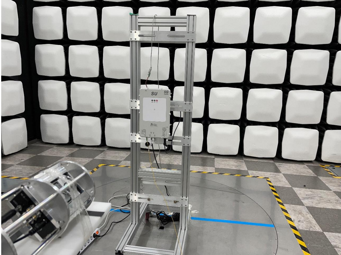
Radiated Test Setup Photo – Spurious (WR-08 Horn Antenna, 45°)
