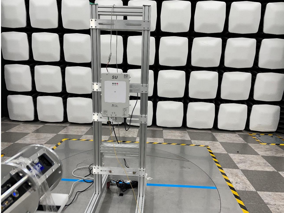
Radiated Test Setup Photo – Spurious (WR-05 Horn Antenna, 45°)
