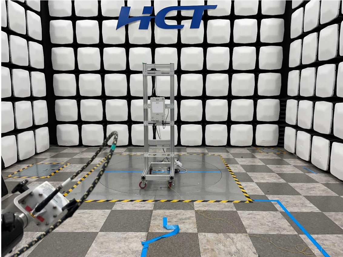
Radiated Test Setup Photo –Spurious (Horn Antenna 18 GHz ~ 40 GHz, 45°)
