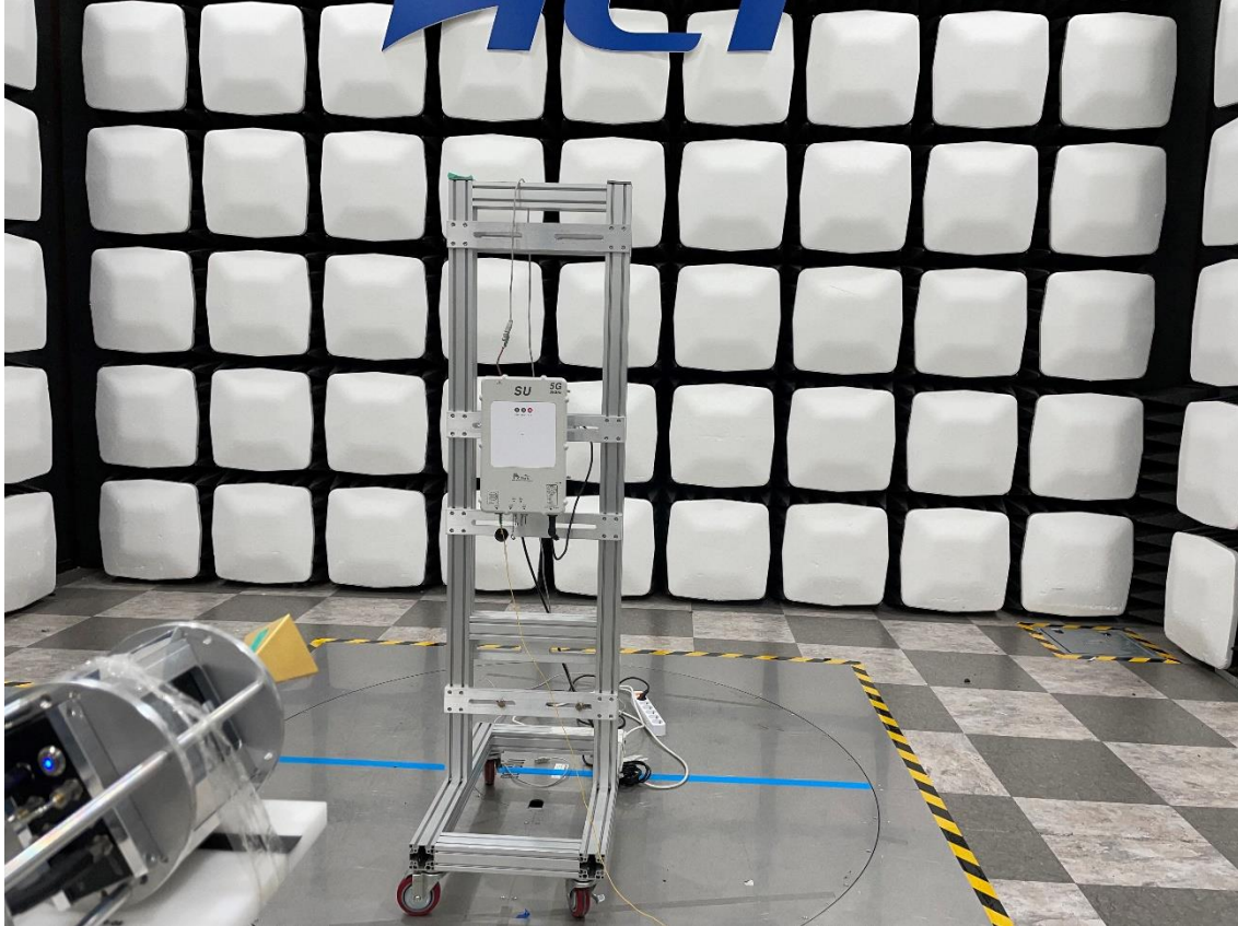
Radiated Test Setup Photo – Spurious (WR-19 Horn Antenna, 45°)
