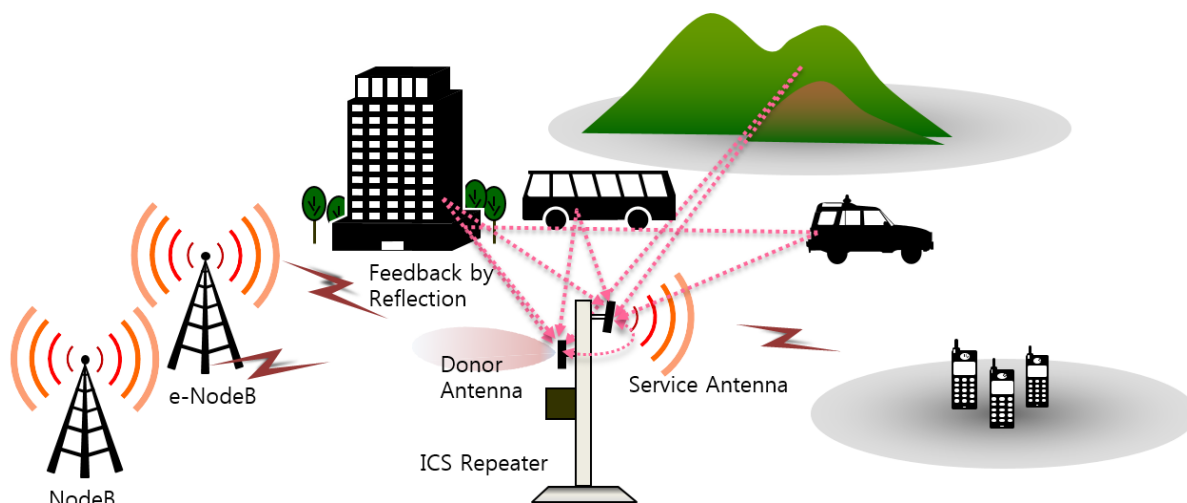
Figure 1. ICS Repeater Service Application Network
