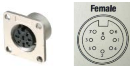
Figure 5. RET Port Connector(SU-20SPR-8S) Pin Map
