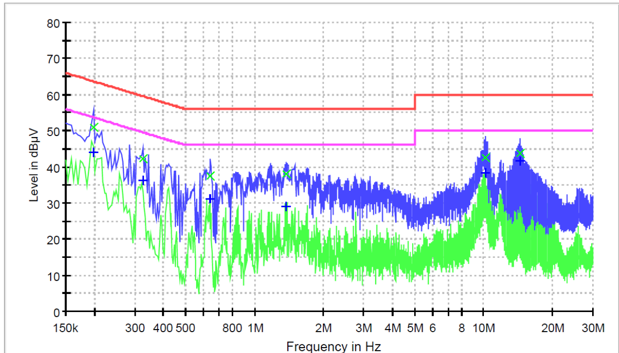
Plots No. 9: AC Mains Conducted Emission _ AC 120V/60Hz _ High Channel _ Line
