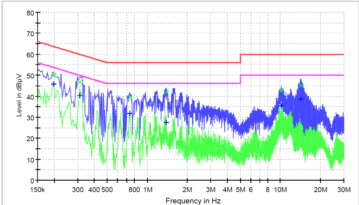
Plots No. 10: AC Mains Conducted Emission _ AC 120V/60Hz _ High Channel _ Neutral
