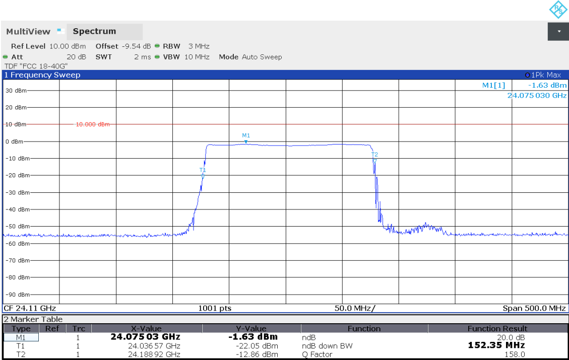
Plots No. 10: 20dB Bandwidth, Horizontal / Vertical Polarization
