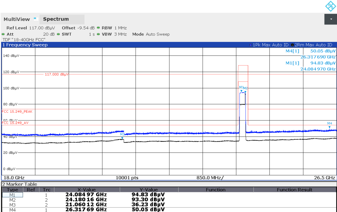
Plots No. 3: 18 GHz to 26.5 GHz, Horizontal / Vertical Polarization
