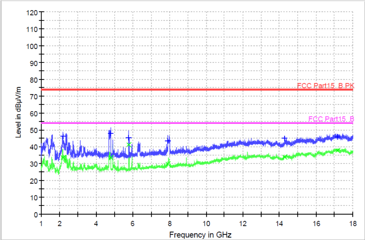
Plots No. 2: 1 GHz to 18 GHz, Horizontal / Vertical Polarization
