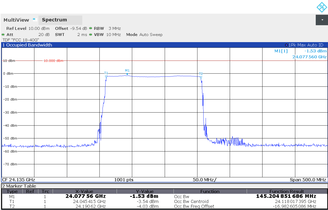
Plots No. 9: 99% Occupied Bandwidth, Horizontal / Vertical Polarization
