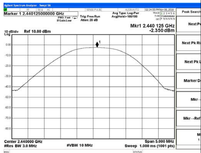
Channel 19 / 2440 MHz
