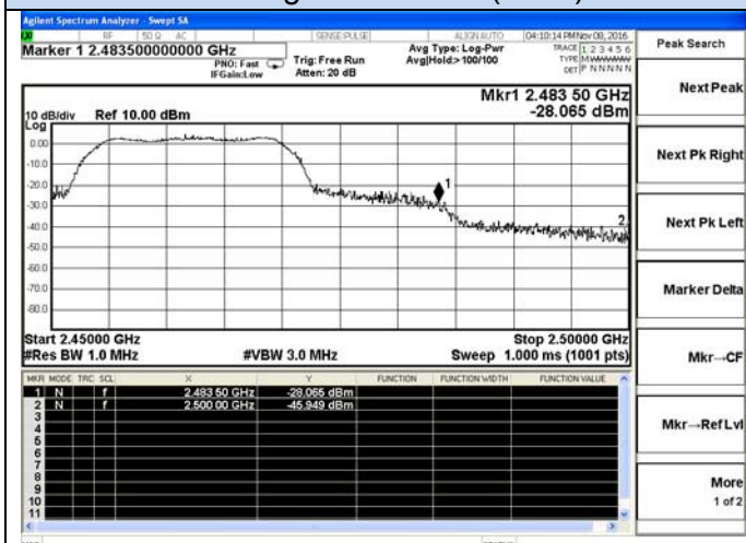
802.11g High channel(Peak)
