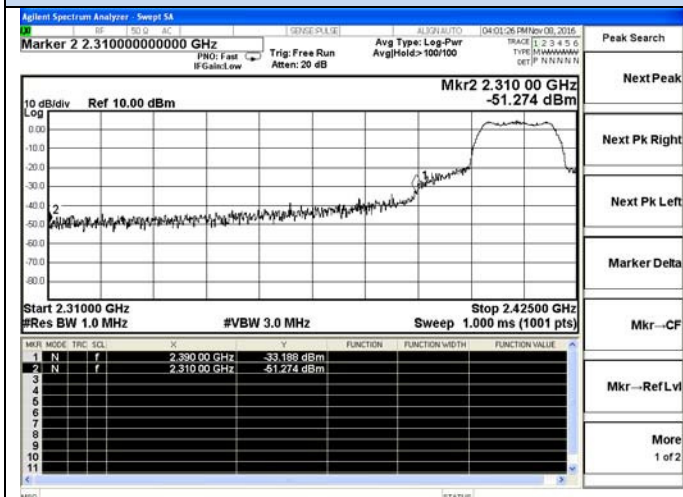
802.11g Low channel(Peak)
