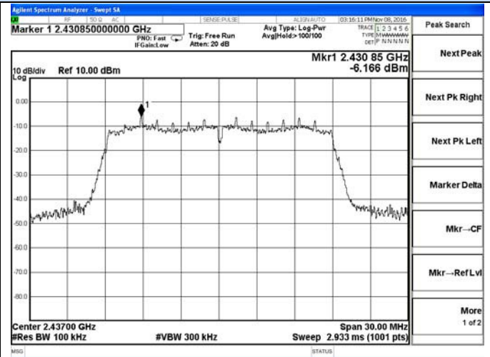
Channel 6 / 2437 MHz
