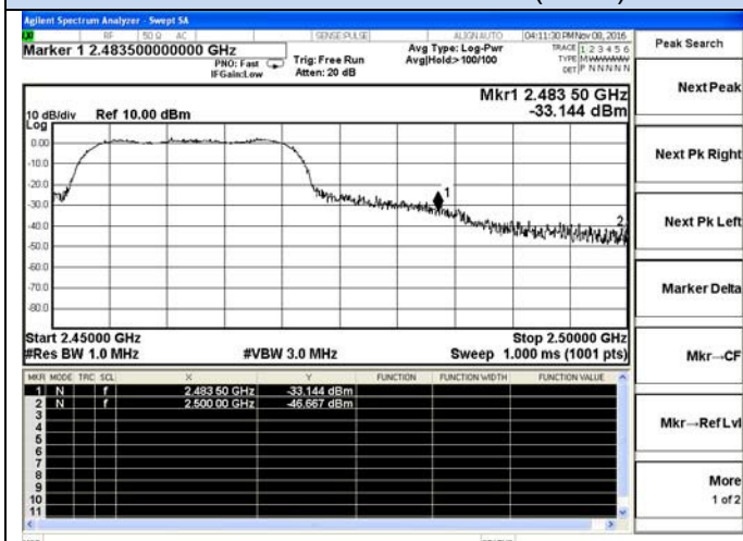
802.11n-HT20 High channel(Peak)
