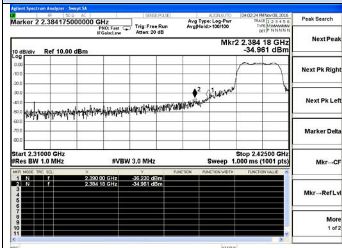
802.11n-HT20 Low channel(Peak)
