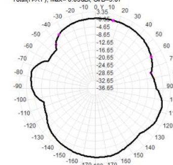
Total(H-XY), Max= 0.09dBi, CirD=9.07
