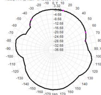
Total(H-XY), Max= 0.12dBi, CirD=9.11
