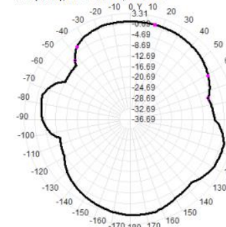
Total(H-XY), Max= 0.19dBi, CirD=9.65
