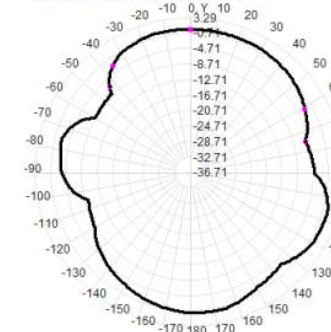
Total(H-XY), Max= 0.25dBi, CirD=9.84
