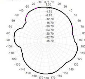
Total(H-XY), Max= 0.31dBi, CirD=9.90
