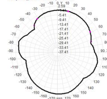
Total(H-XY), Max=-0.78dBi, CirD=8.75
