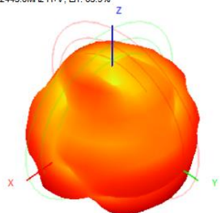
2445.0MHz H+V, Eff: 65.9%
