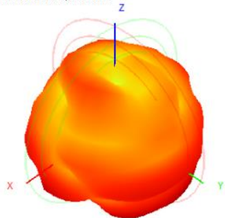
2460.0MHz H+V, Eff: 64.3%
