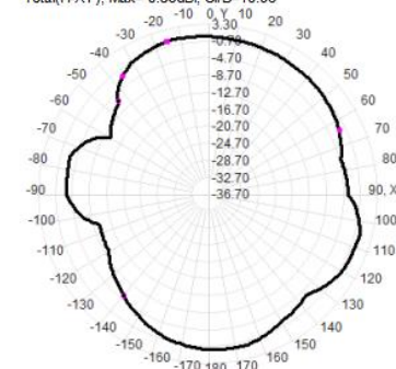
Total(H+V), Max= 0.56dBi, CirD=10.86
