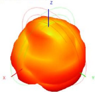
2465.0MHz H+V, Eff: 63.9%
