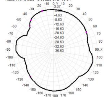
Total(H-XY), Max= 0.60dBi, CirD=10.64
