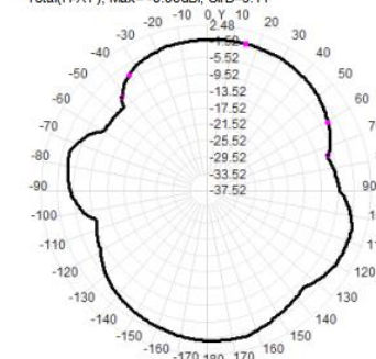
Total(H-XY), Max= -0.86dBi, CirD=9.11
