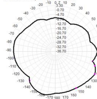
2470.0MHz Total(E2-YZ), Max= 3.30dBi
