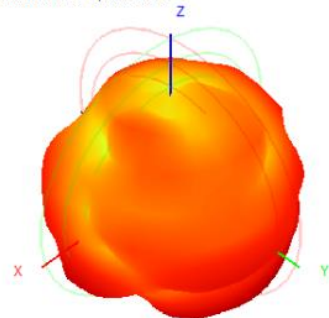
2420.0MHz H+V, Eff: 54.3%
