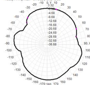
Total(H-XY), Max= 0.18dBi, CirD=9.35
