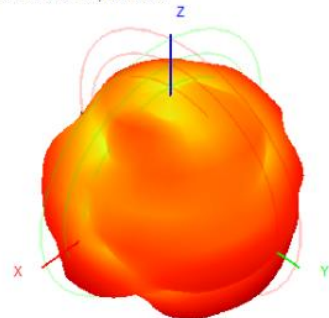
2425.0MHz H+V, Eff: 55.2%
