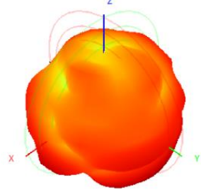
2410.0MHz H+V, Eff: 53.8%
