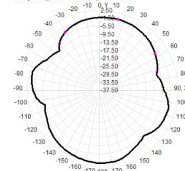
Total(H-XY), Max=-0.82dBi, CirD=8.83
