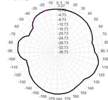
Total(H-XY), Max= 0.35dBi, CirD=10.00
