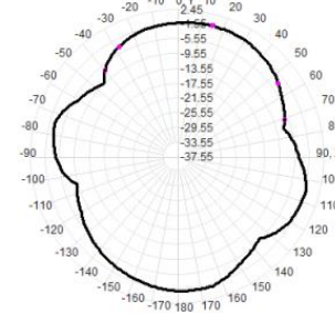
Total(H-XY), Max= -0.77dBi, CirD=8.85
